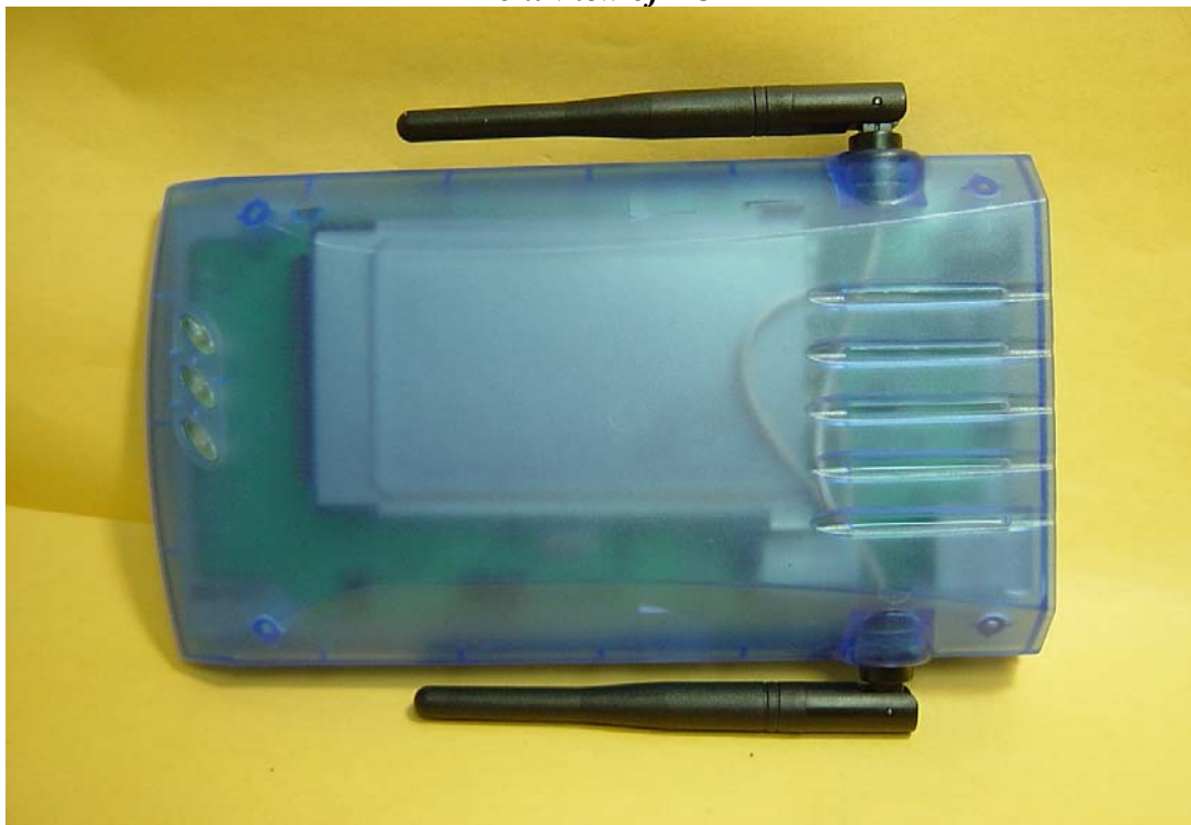
Front View of EUT
