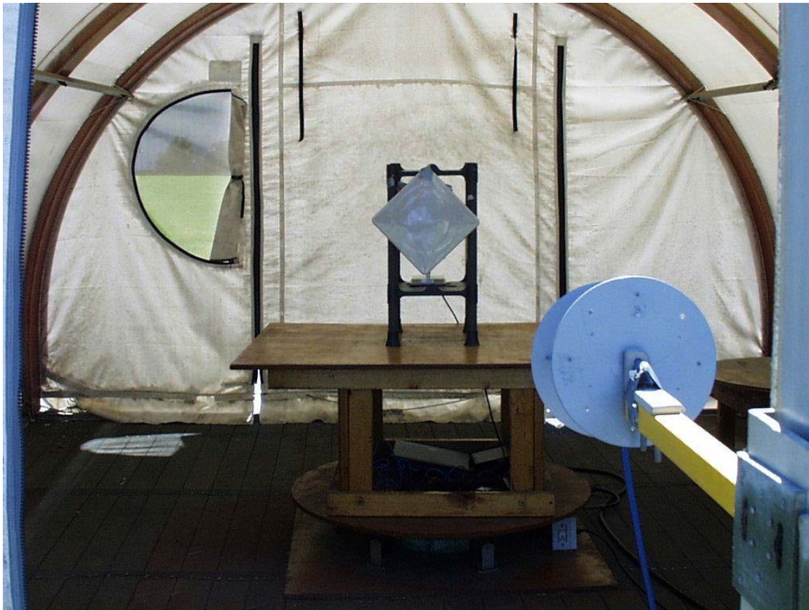
MAR Antenna 23 dBi panel
