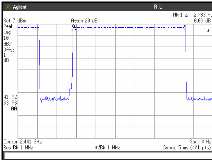
Dwell Time GFSK Mode
