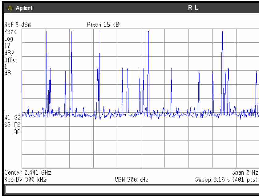
Number of Pulses in GFSK Mode
