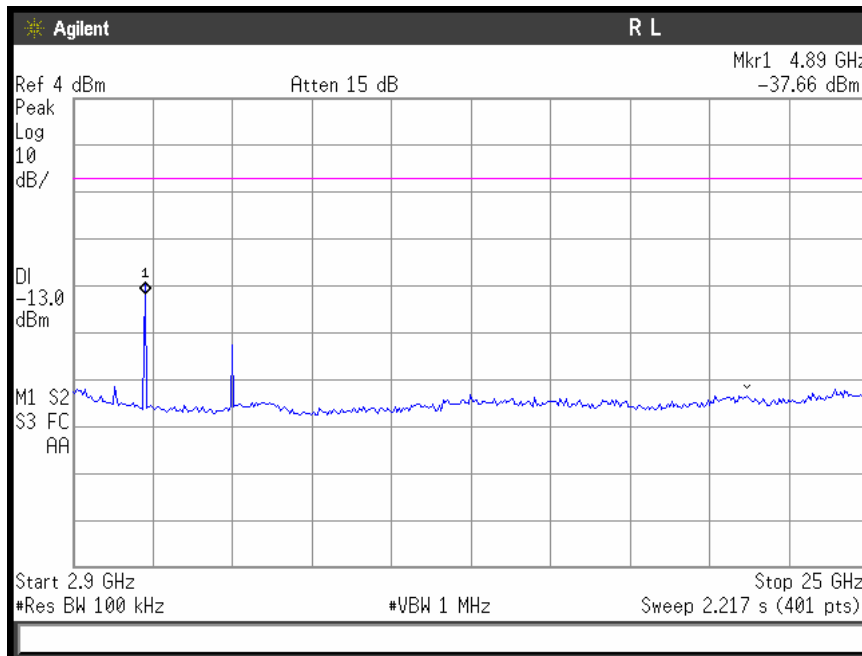
Mid channel (2441 MHz) Spurious Emission 2.9 GHz - 25 GHz 8PSK Mode
