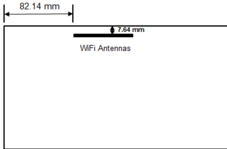
Antenna Location - Bottom View
