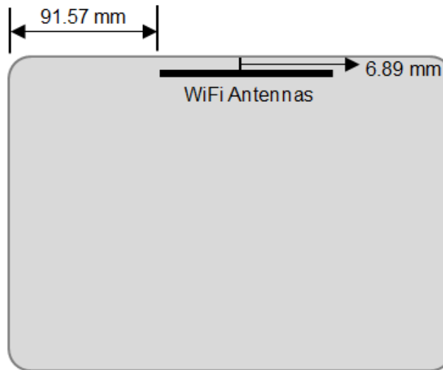
Antenna Location – Bottom View
