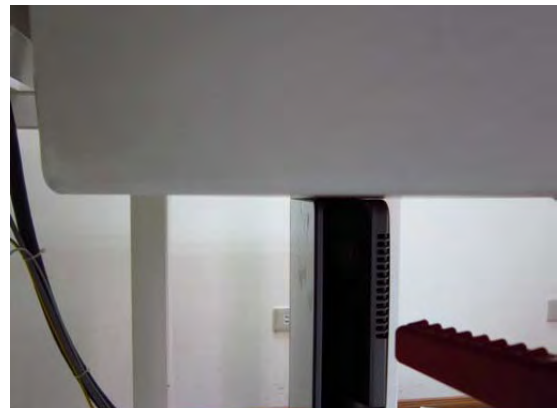
Fig.4 EUT Left to flat phantom
