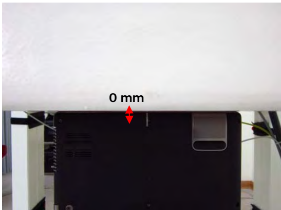
Fig.4 EUT Left to flat phantom
