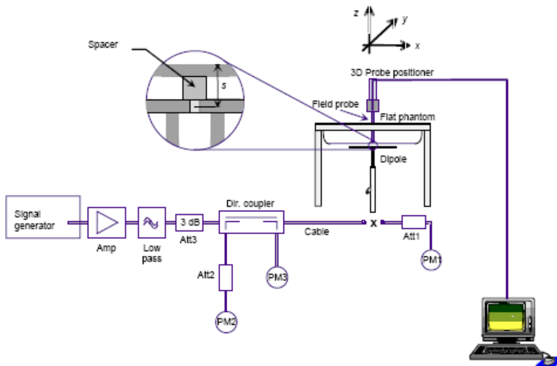
Figure 9.1 Dipole Validation Test Setup
