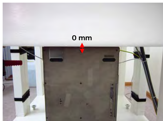
Fig.5 EUT Edge 2 mode to flat phantom
