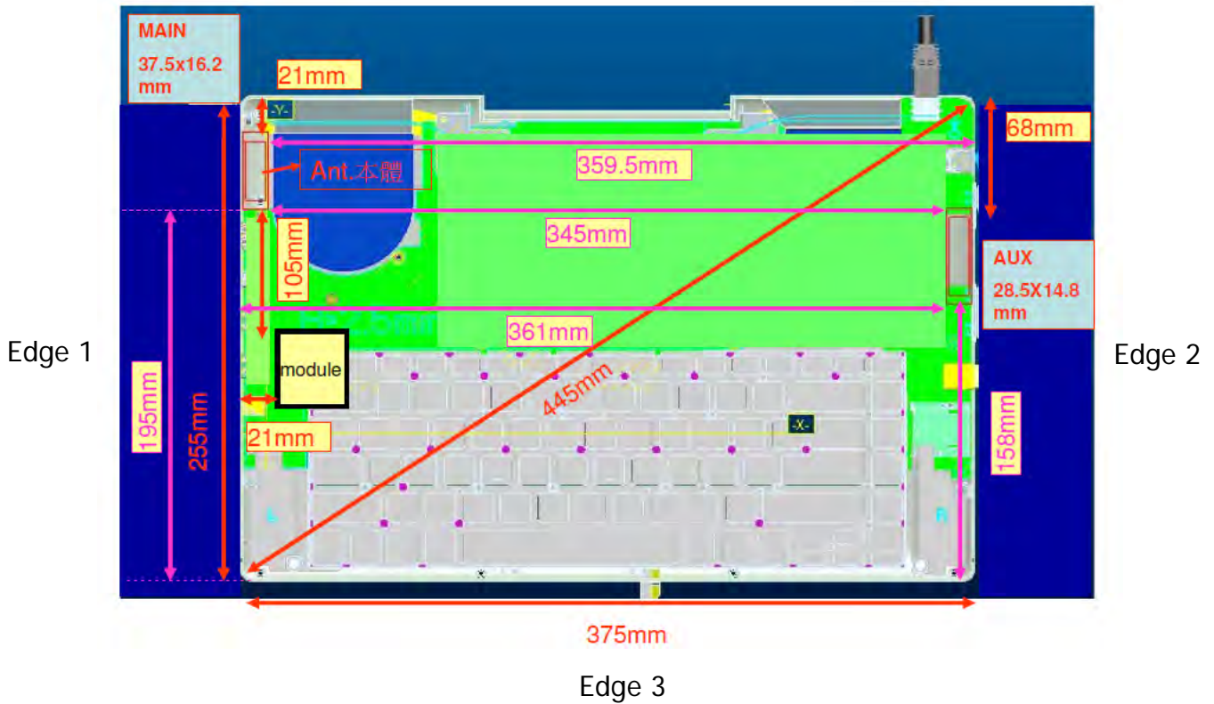
Fig.6 Antenna position of EUT
