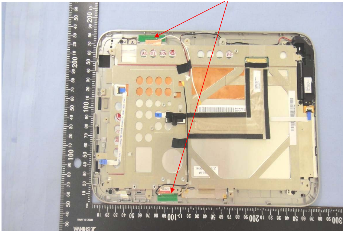
WLAN & BT Antenna
