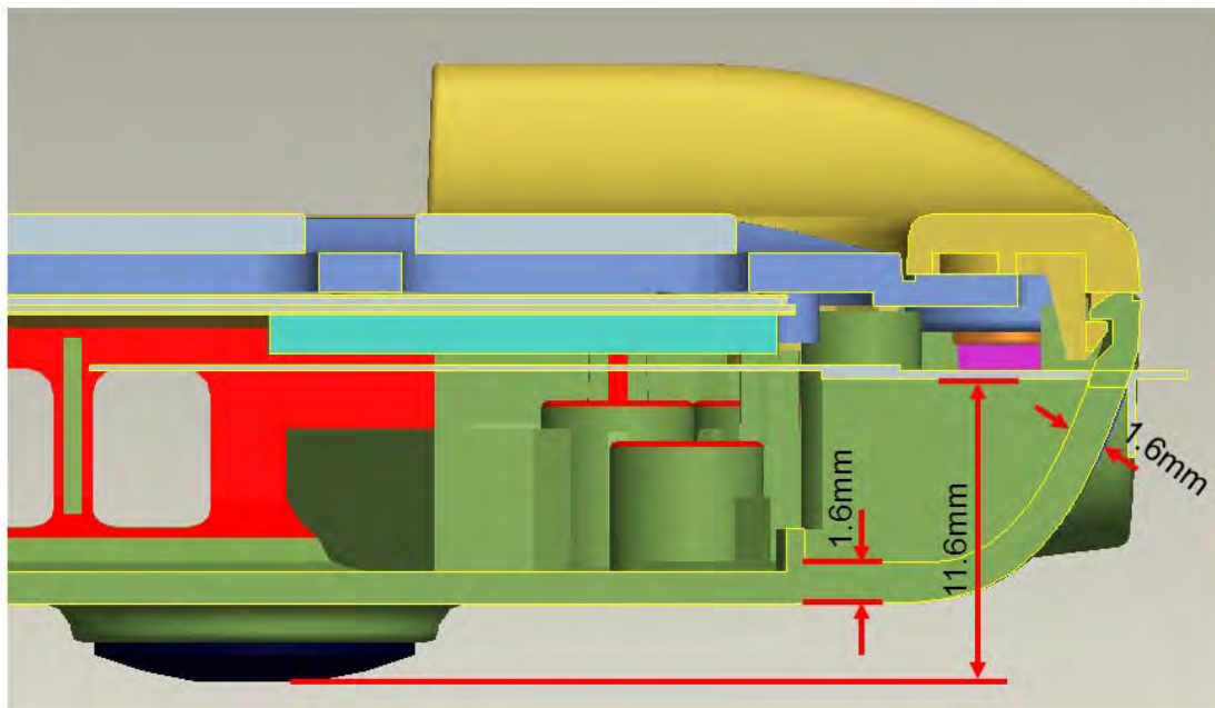
Fig.7 Aux Antenna position of EUT
