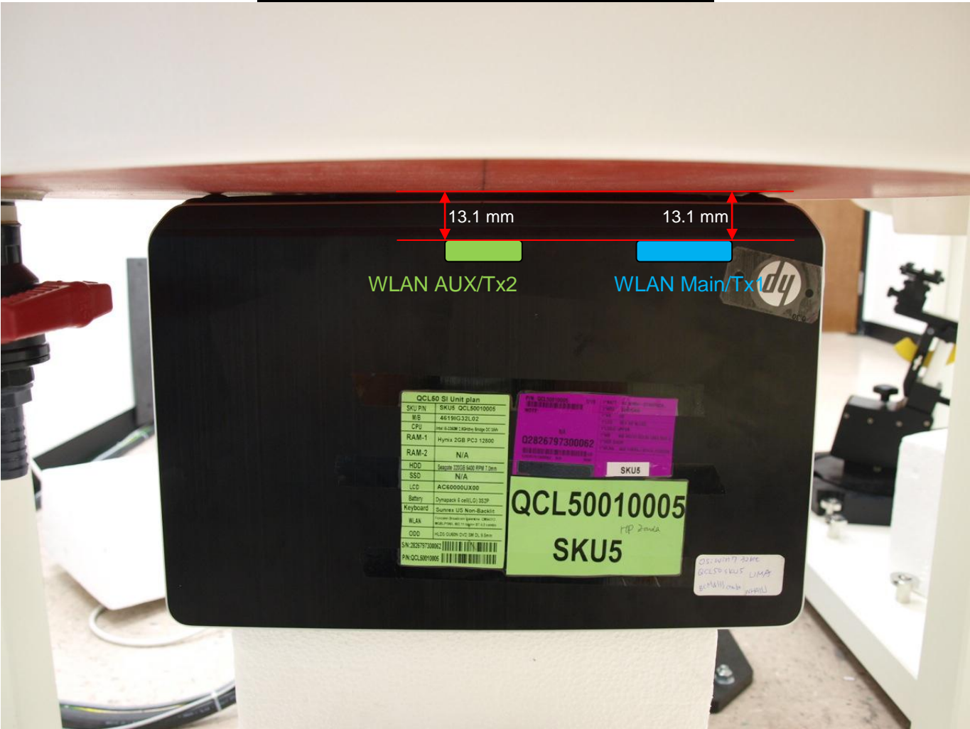
Lap-held with display open at 90° to the keyboard
