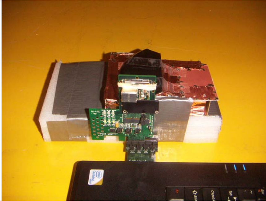
RADIATED CLOSE UP FRONT PHOTO
