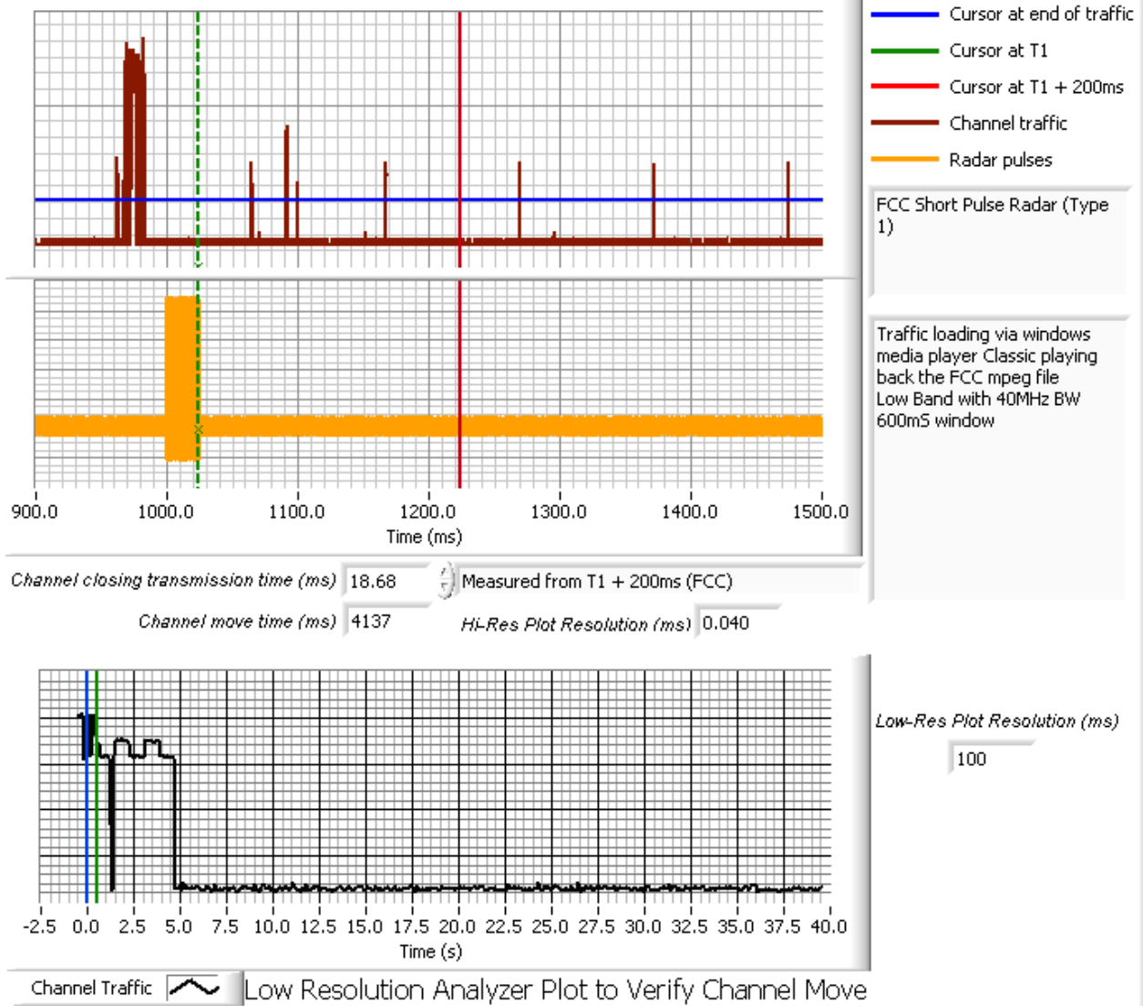
Figure 7: Channel Closing Time, 40MHz BW (Close-Up Showing Radar Burst and Subsequent Transmissions at 5310 MHz)
