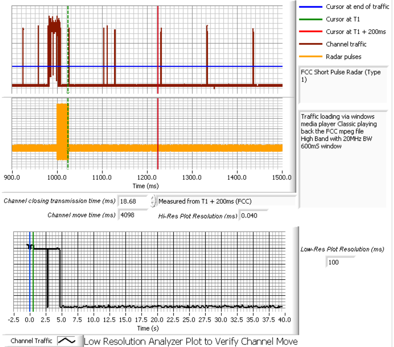
Figure 5: Channel Closing Time, 20MHz BW (Close-Up Showing Radar Burst and Subsequent Transmissions at 5600 MHz)
