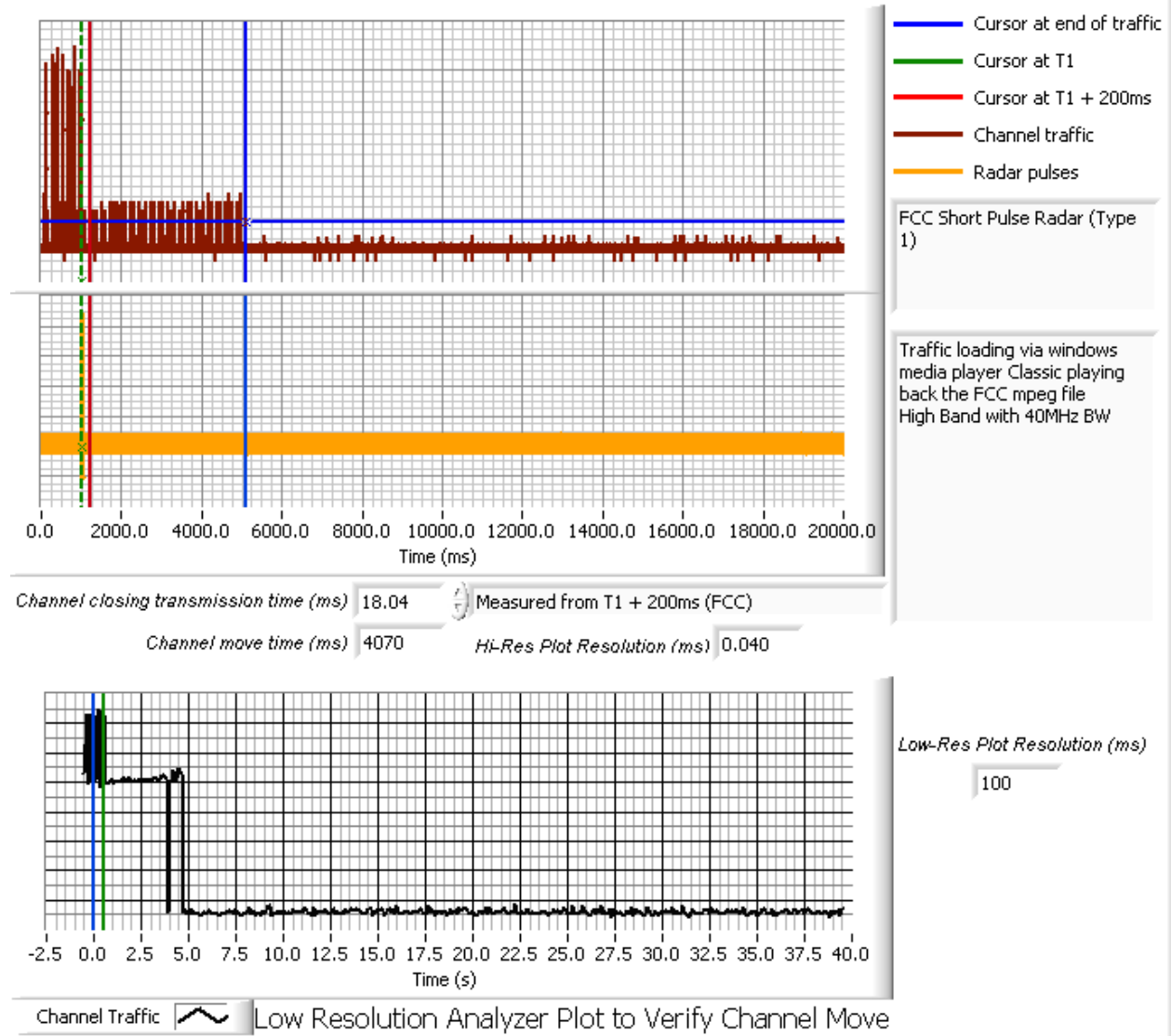
Figure 8: Channel Closing Time and Channel Move Time, 40MHz BW (40 second plot, at 5590 MHz)
