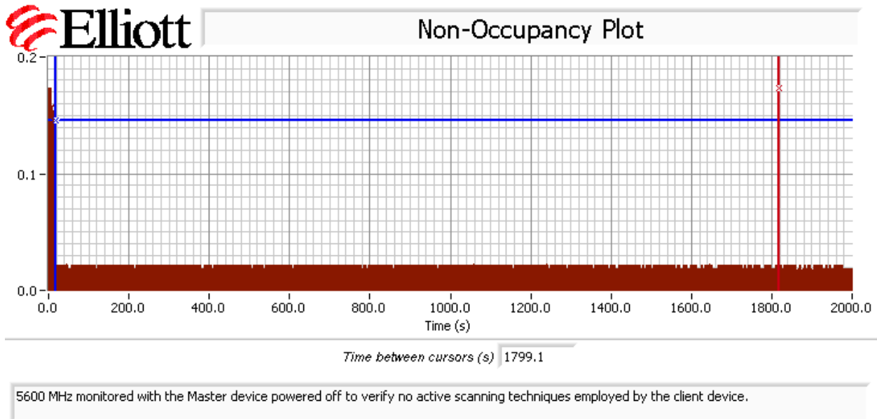
Figure 10: Confirmation of Passive Scanning For Client Devices (Non-associated Test)
