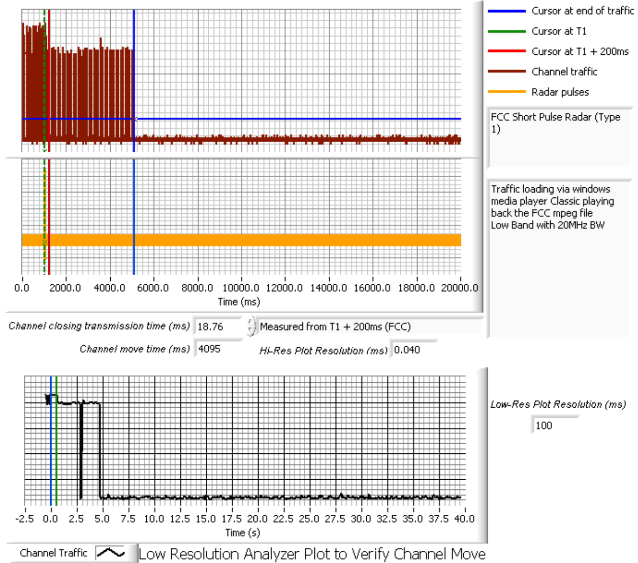
Figure 2: Channel Closing Time and Channel Move Time, 20MHz BW (40 second plot at 5300 MHz)
