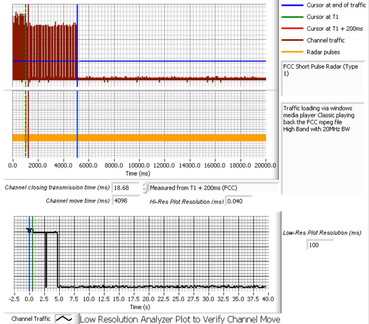
Figure 4: Channel Closing Time and Channel Move Time, 20MHz BW (40 second plot, at 5600 MHz)
