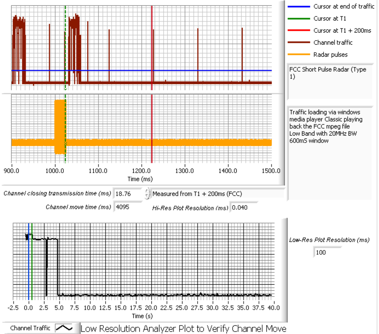
Figure 3: Channel Closing Time, 20MHz BW (Close-Up Showing Radar Burst and Subsequent Transmissions at 5300 MHz)
