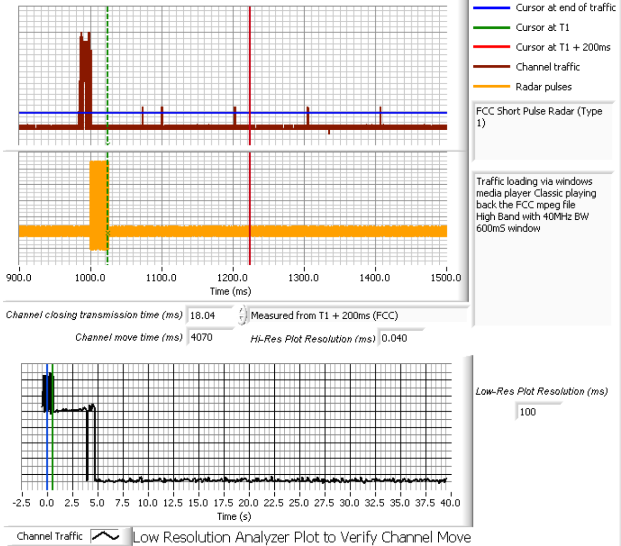
Figure 9: Channel Closing Time, 40MHz BW (Close-Up Showing Radar Burst and Subsequent Transmissions at 5590 MHz)
