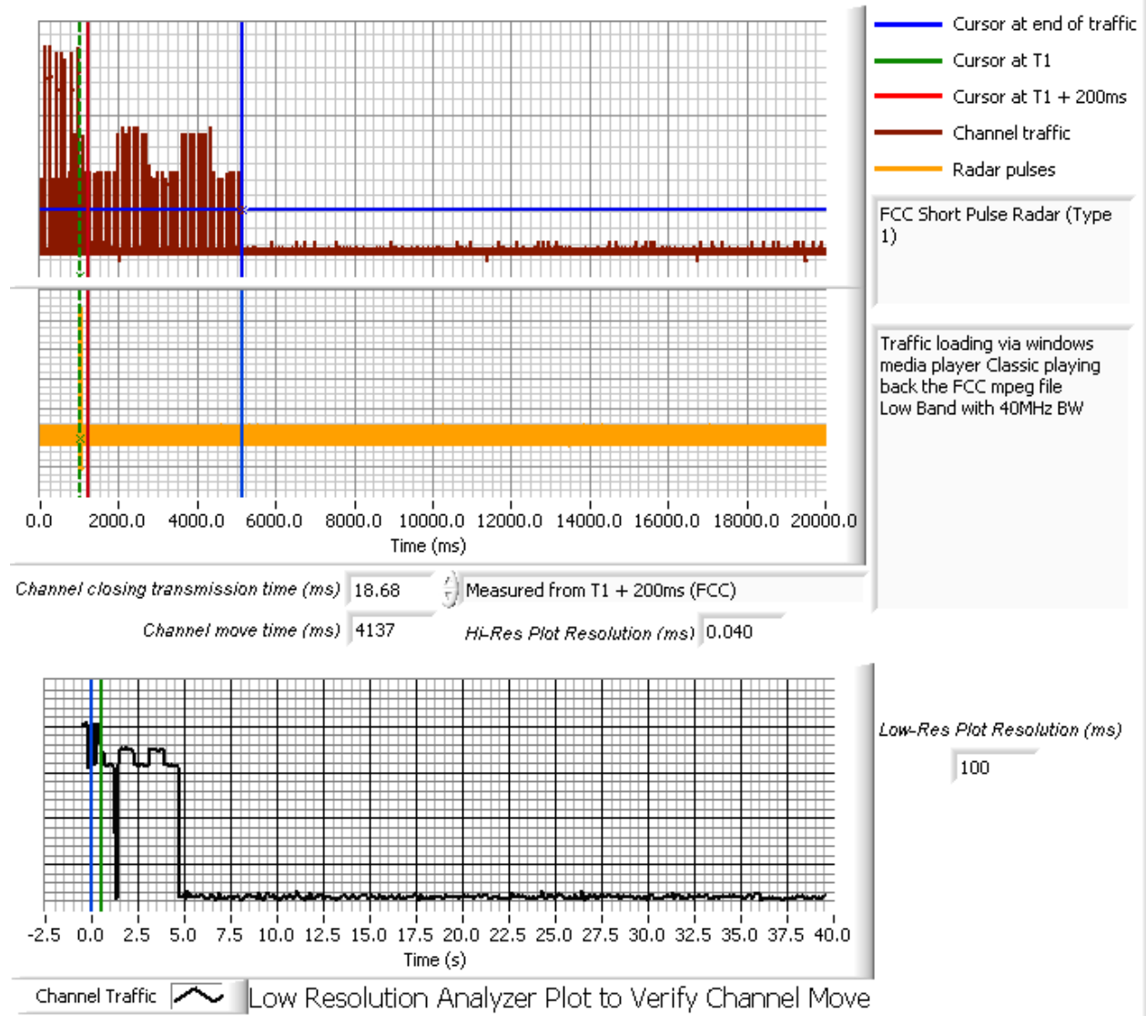
Figure 6: Channel Closing Time and Channel Move Time, 40MHz BW (40 second plot, at 5310 MHz)
