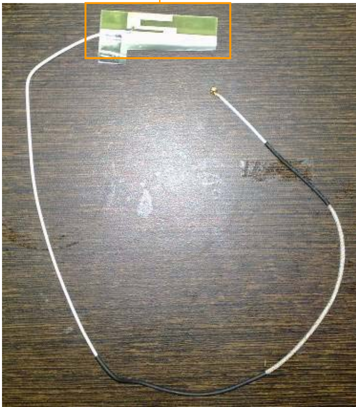
Tx1 Antenna
