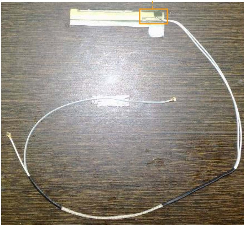
Tx1 Antenna
