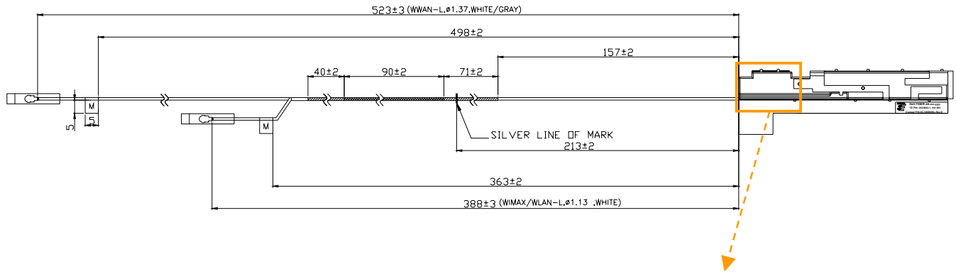
Tx1 Antenna
