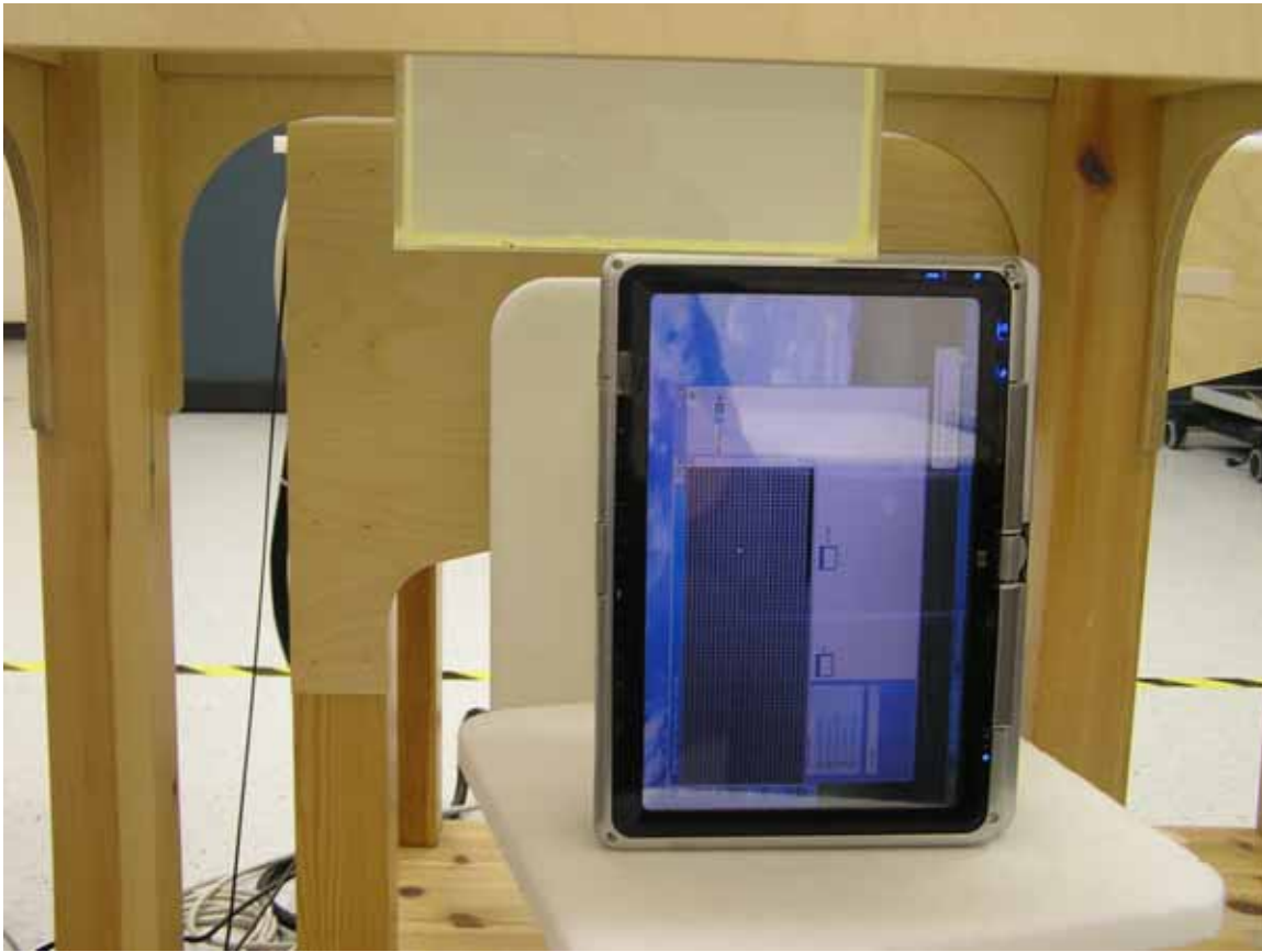
Photo 2. Tablet position, main antenna, right side
