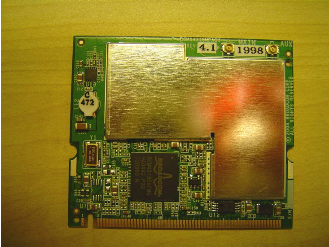
WLAN – Top view with shielding
