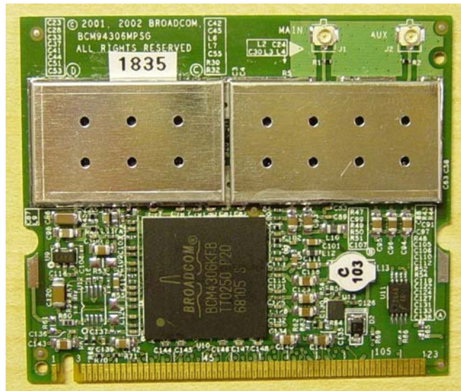
Photo 2. Card top
