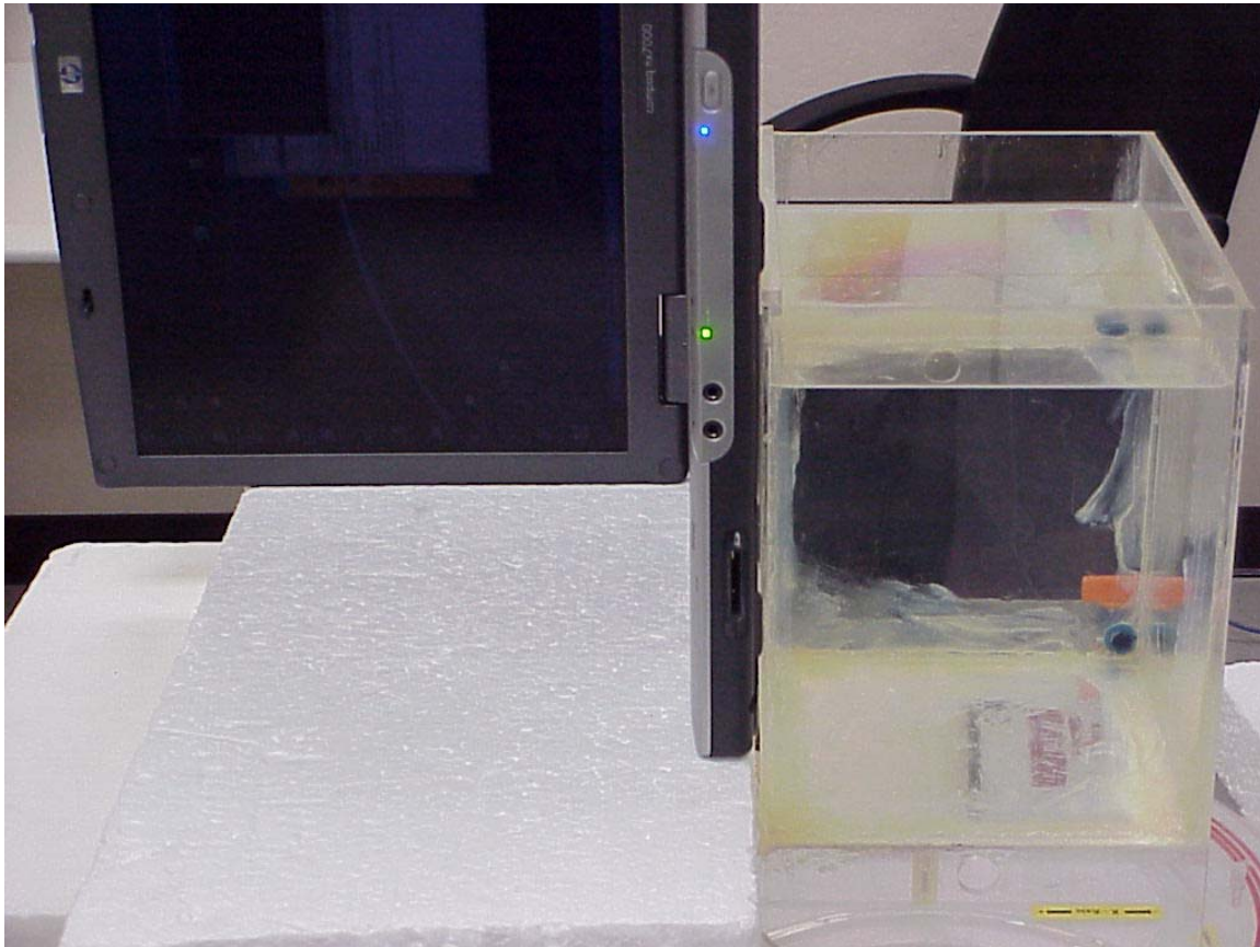
Photo 11. Left antenna lap position
