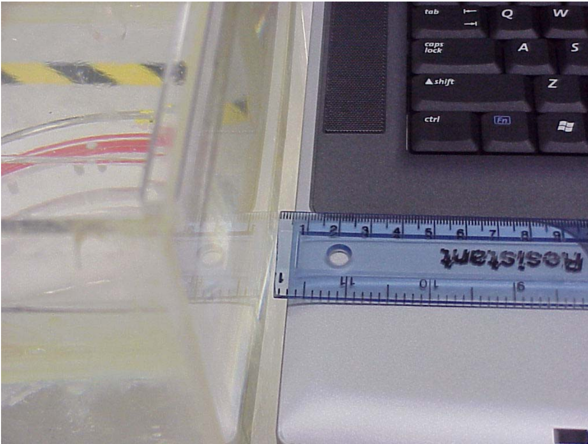
Photo 10. Left antenna bystander position distance
