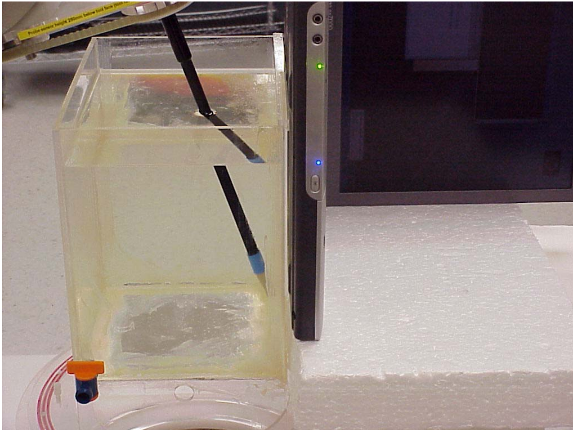
Photo 8. Right antenna lap position
