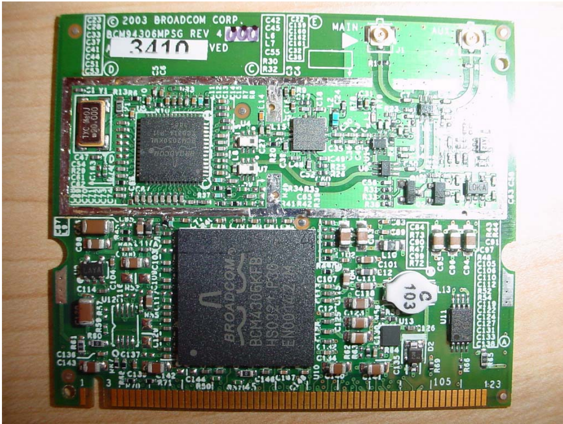
WLAN Model# BCM94306MPSG Top view - unshielded
