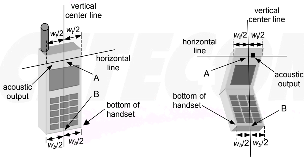
Figure 1a – Handset vertical and horizontal reference lines – fixed case
