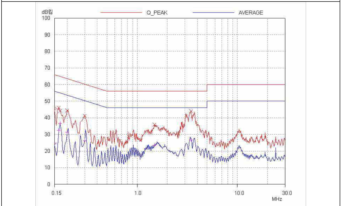
NEUTRAL LINE
