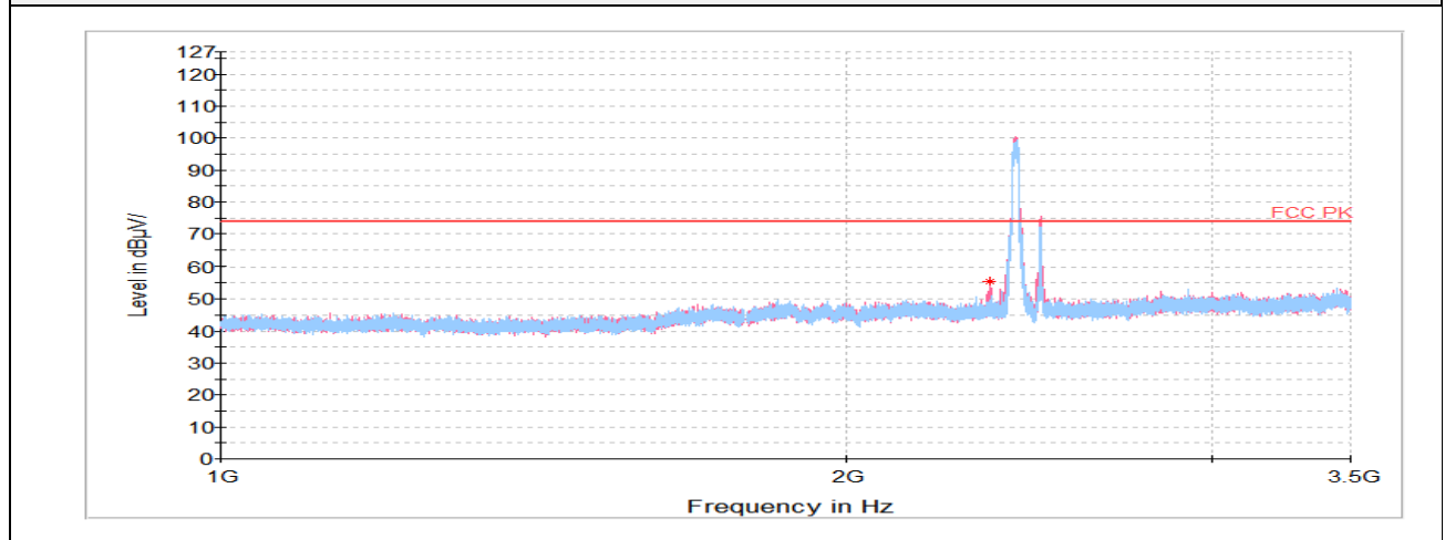
Horizontal/Vertical for 1 GHz ~ 3.5 GHz
