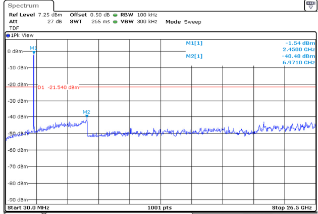
802.11n HT20 / 6 ch.
