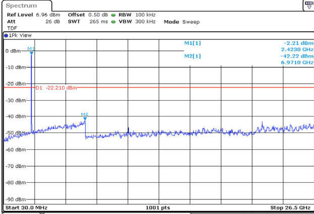
802.11n HT20 / 1 ch.
