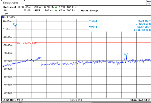
802.11b / 1 ch.
