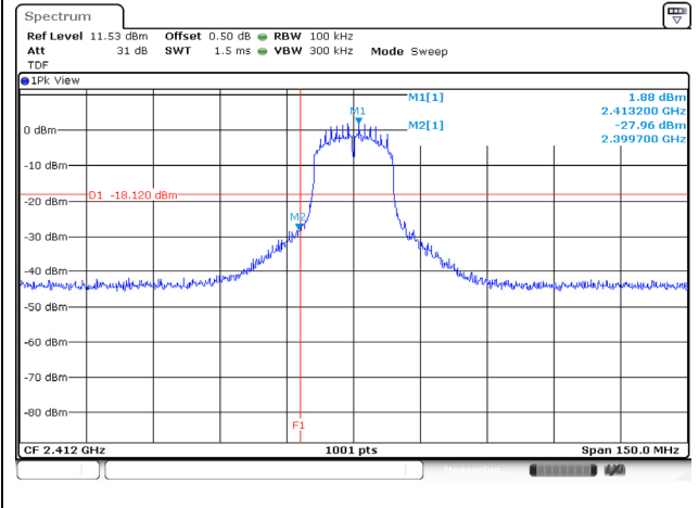
802.11n HT20 / 1 ch.
