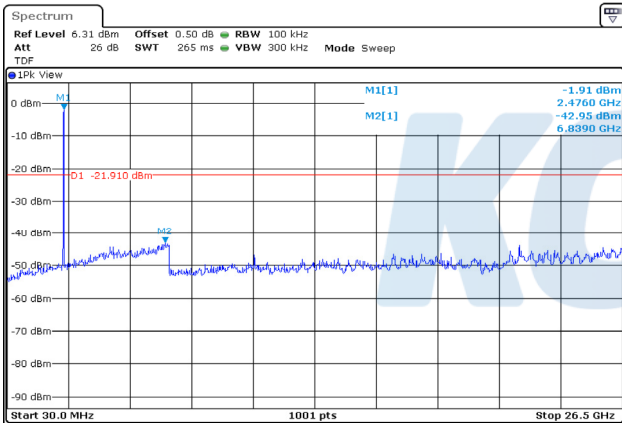
802.11n HT20 / 11 ch.
