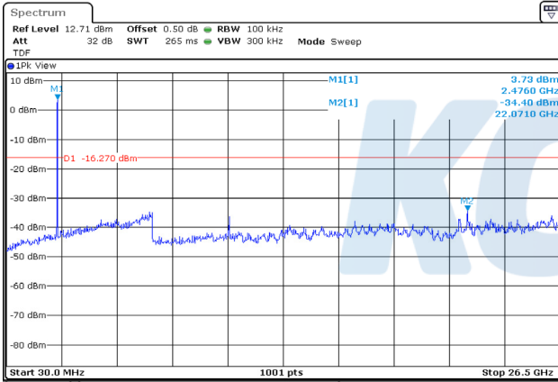
802.11b / 11 ch.
