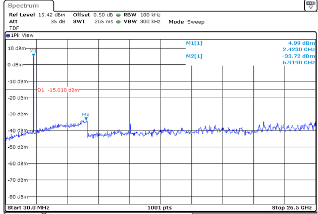
802.11b / 6 ch.
