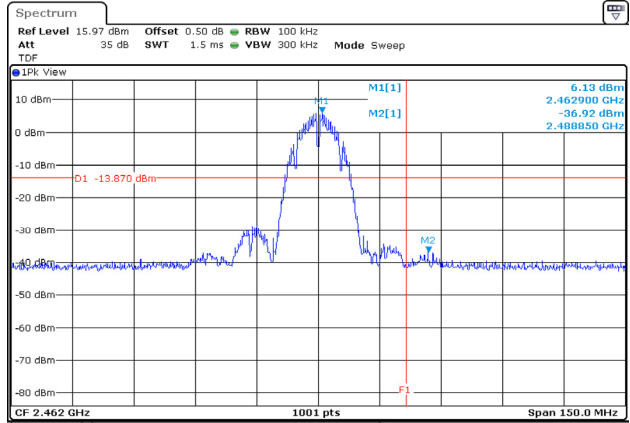
802.11b / 11 ch.
