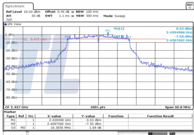
802.11g / 2 437 MHz
