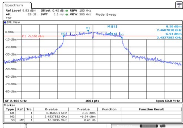
802.11g / 2 462 MHz
