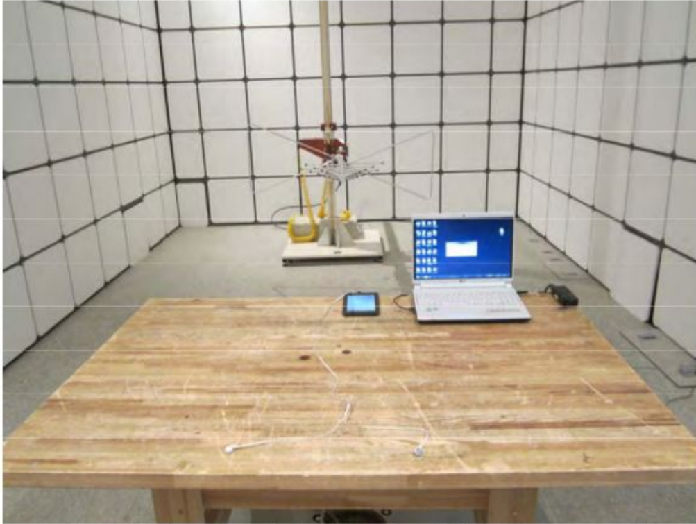
Radiated Emissions Below 1 GHz- Front View(Up & Down mode)
