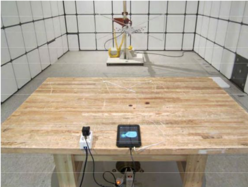
Radiated Emissions Below 1 GHz- Front View(Play mode)
