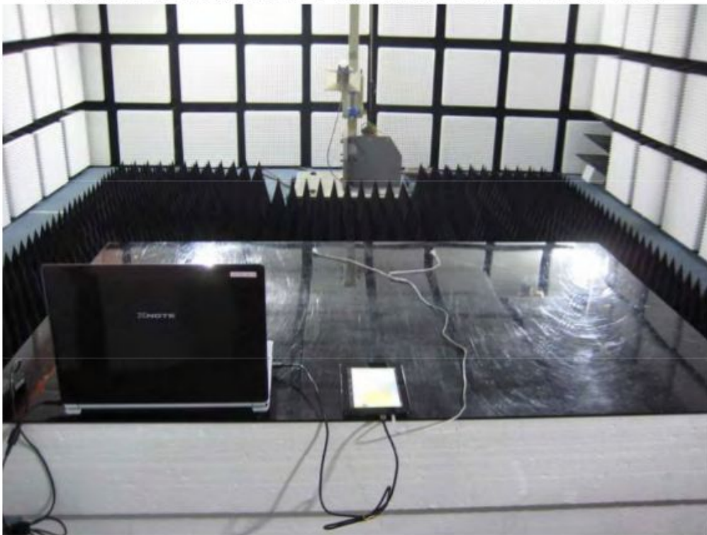
Radiated Emissions Above 1 GHz - Rear View(Up & Down mode)
