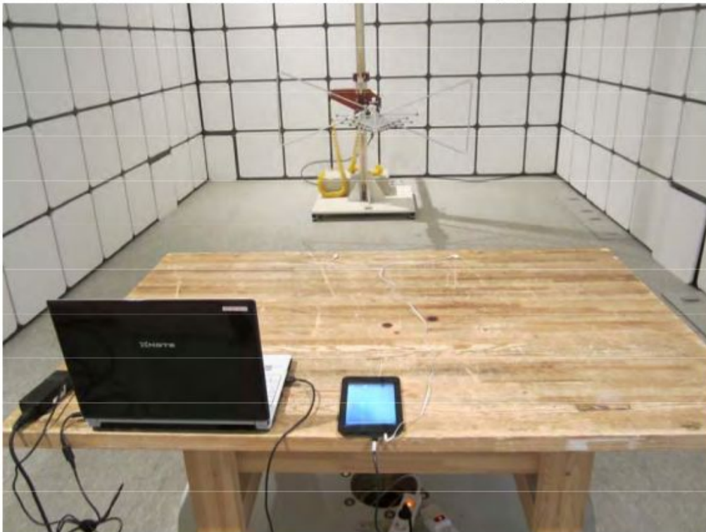
Radiated Emissions Below 1 GHz - Rear View(Up & Down mode)
