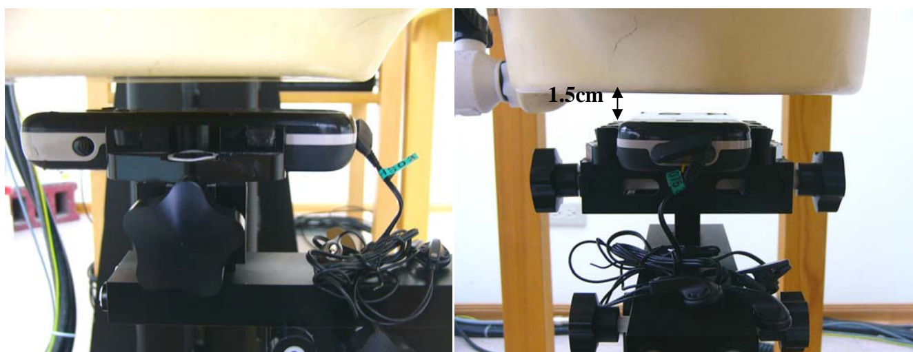
Fig.9 Body worn- EUT back to flat phantom with headset (testing in GPRS Mode)
