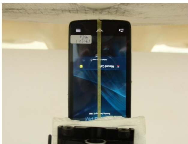
Bottom Side of the DUT with Phantom 1 cm Gap (DUT without Earphone)
