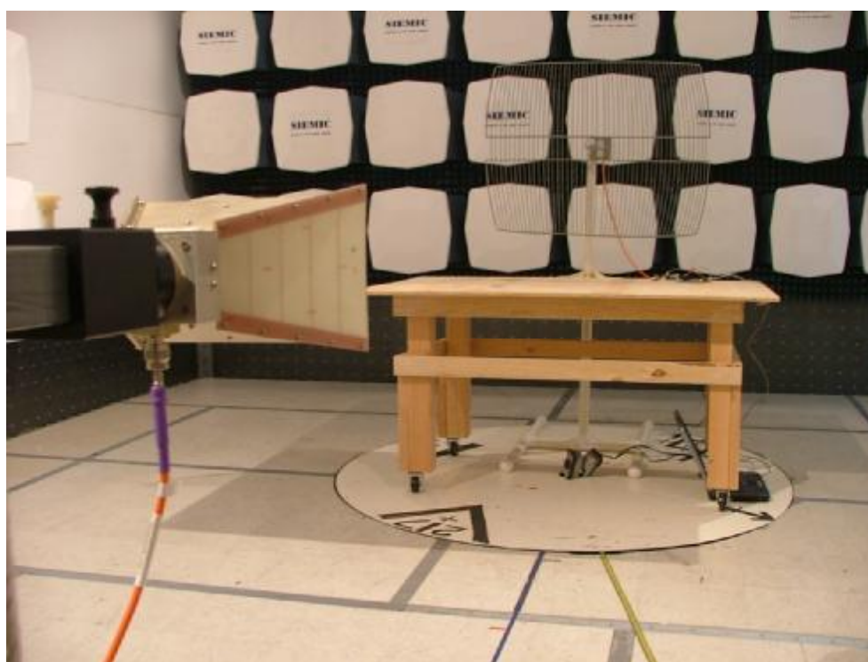
Radiated Emissions Grid Antenna
