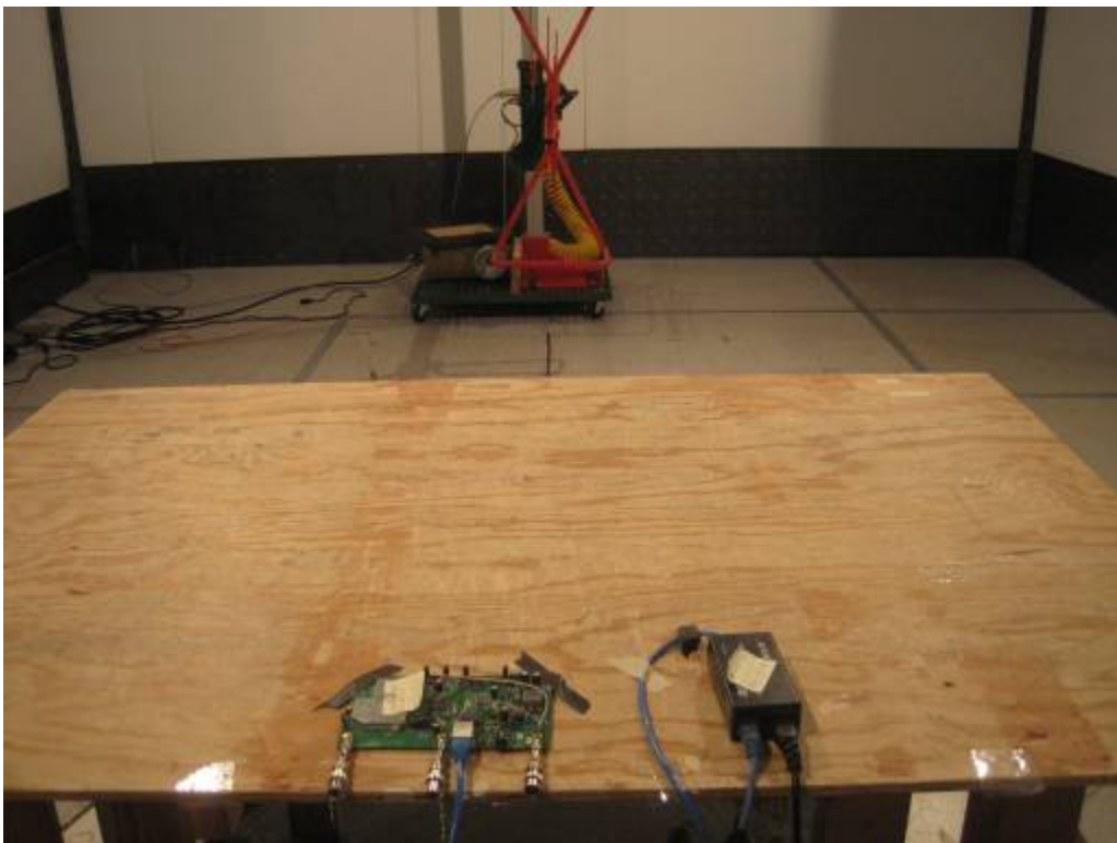
Radiated Emission View with power supply 2(PoE) (<30MHz)
