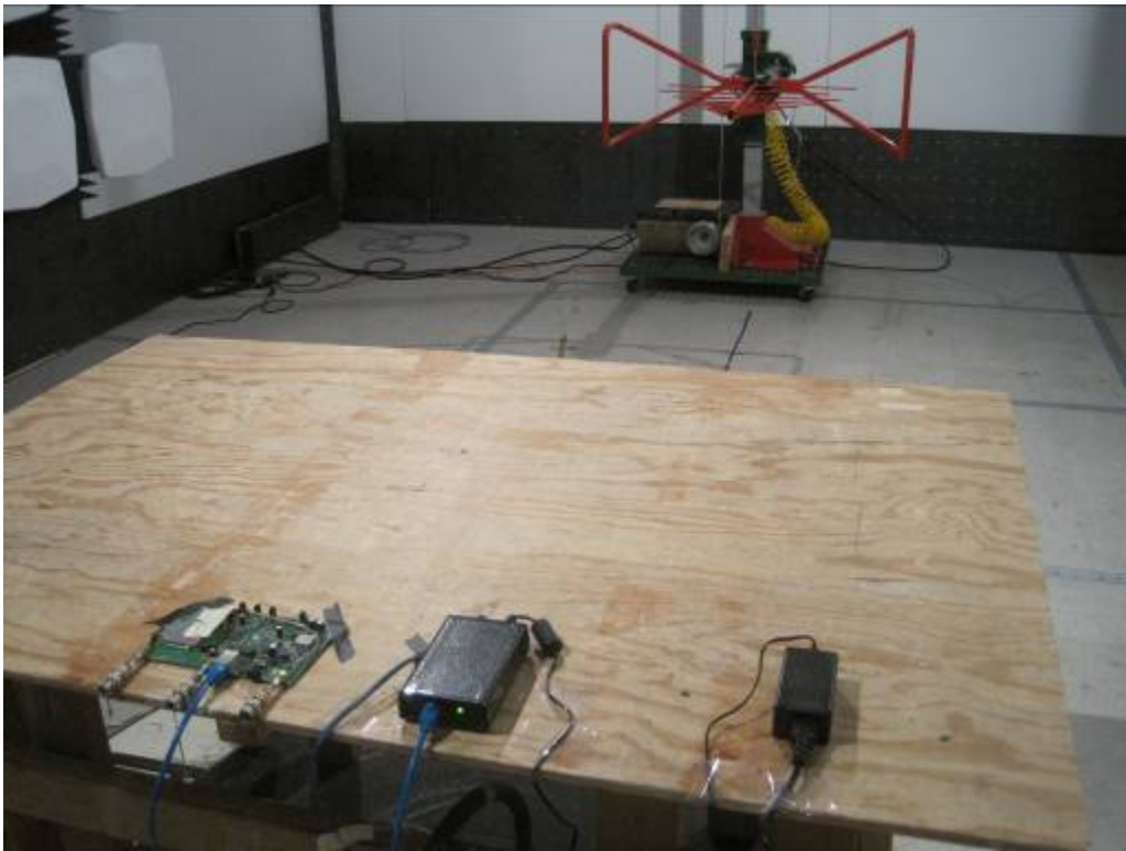
Radiated Emission View with power supply 1(PoE) (<30MHz)
