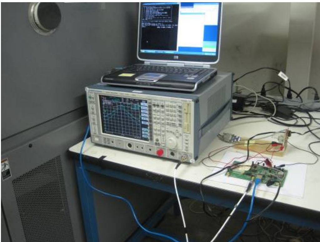
RF conducted Testing Setup
