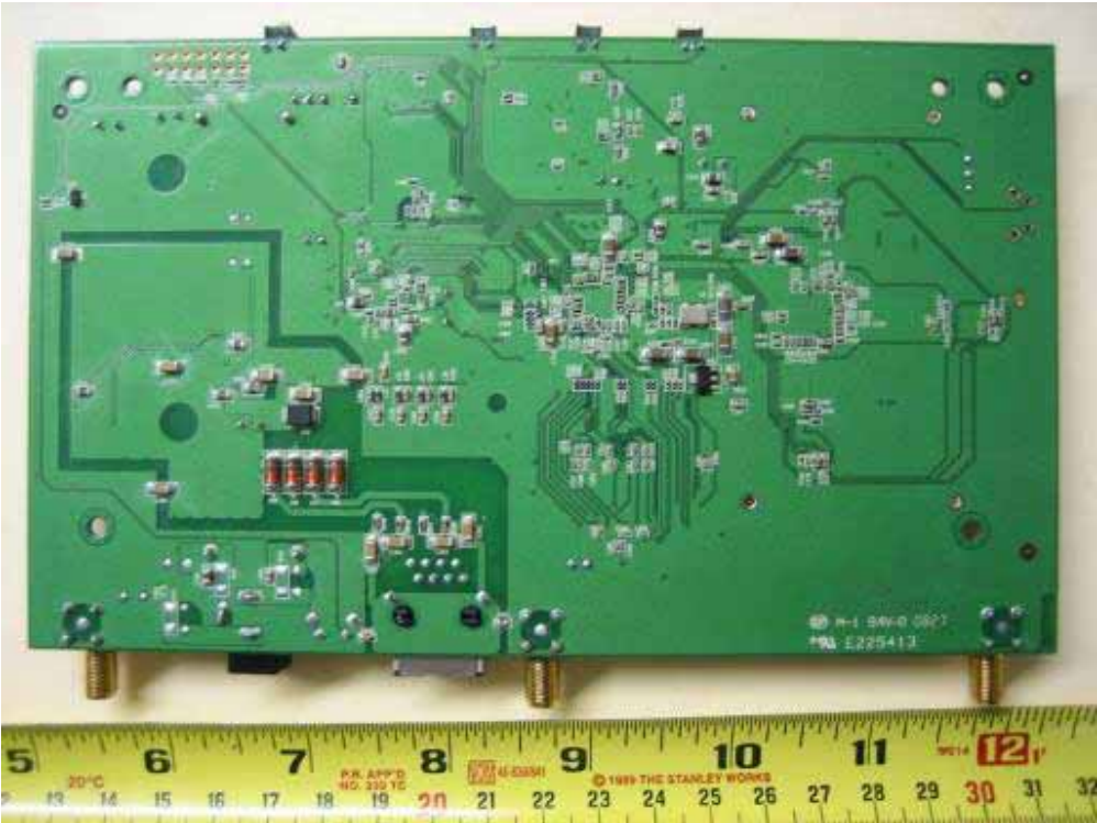
Solder View
