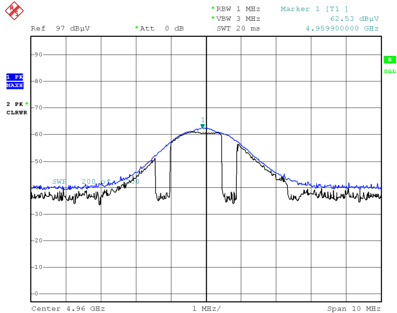
Radiated Spurious Emissions plot – Peak Result (GFSK, Ch.78 2nd Harmonic, H)
