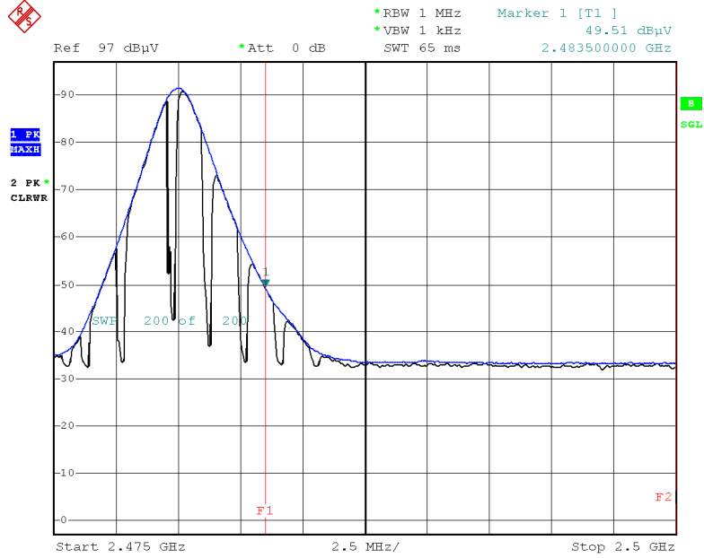
Radiated Restricted Band Edges plot – Average Result (GFSK, Ch.78, Z-H)
