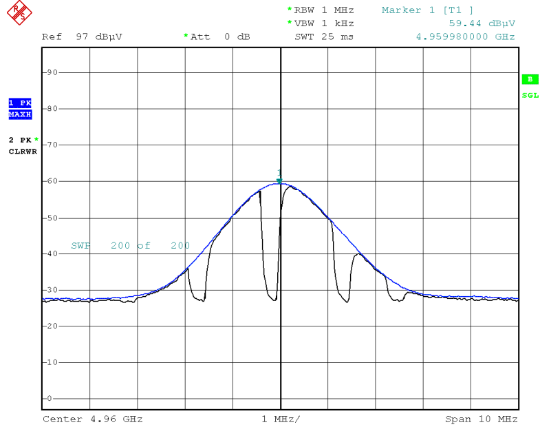
Radiated Spurious Emissions plot – Average Result (GFSK, Ch.78 2nd Harmonic, H)
