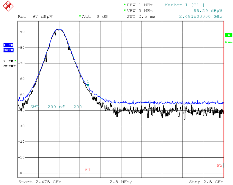
Radiated Restricted Band Edges plot – Peak Result (GFSK, Ch.78, Z-H)
