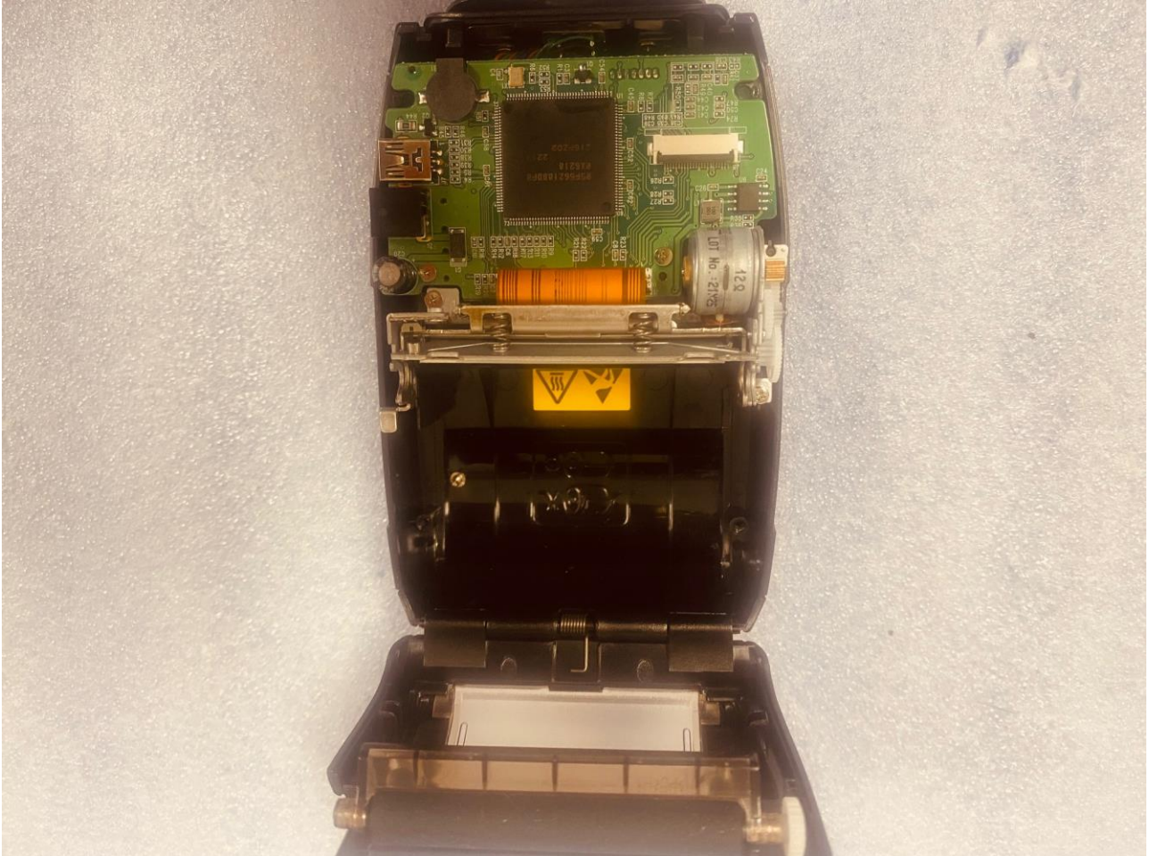
(Assy Main)
