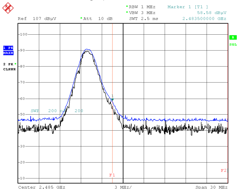
Radiated Restricted Band Edges plot – Peak Result ( \pi/4 DQPSK, Ch.78, Z-H)
