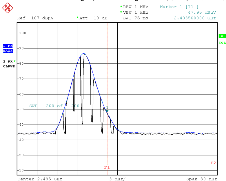
Radiated Restricted Band Edges plot – Average Result ( \pi/4 DQPSK, Ch.78, Z-H)
