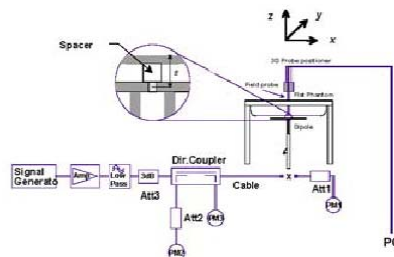
Figure 11.1 Dipole Verification Test Setup
