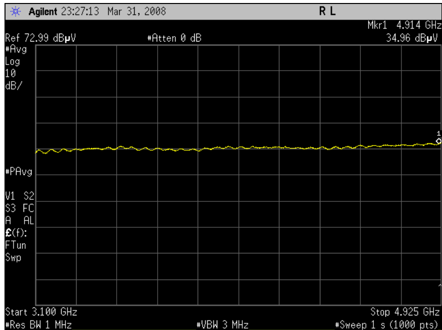
Plot 7. Average, 3100 – 4925 MHz
