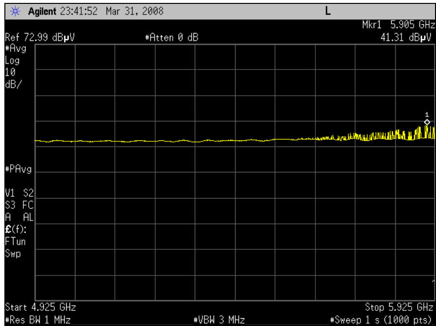
Plot 8. Average, 4925 – 5925 MHz
