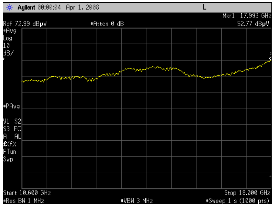
Plot 11. Average, 10600 – 18000 MHz
