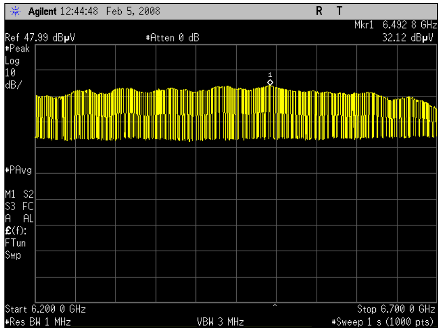
Plot 13. Peak Emissions, 6.2 – 6.7 GHz
