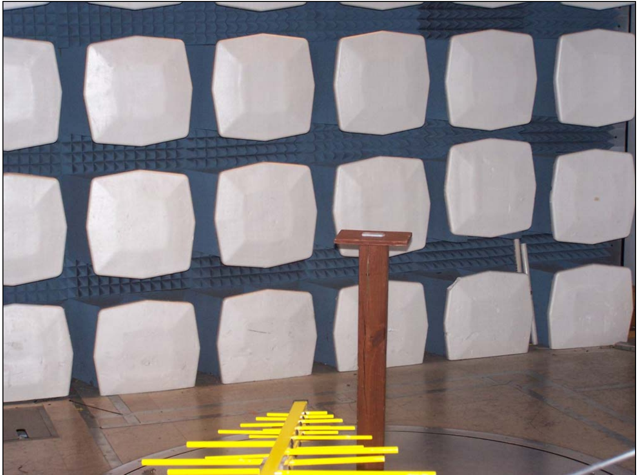
Photograph 5. Radiated Emissions Below 960 MHz, Test Setup
