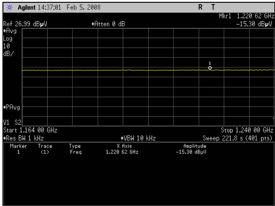
Plot 11. GPS, Band 1
