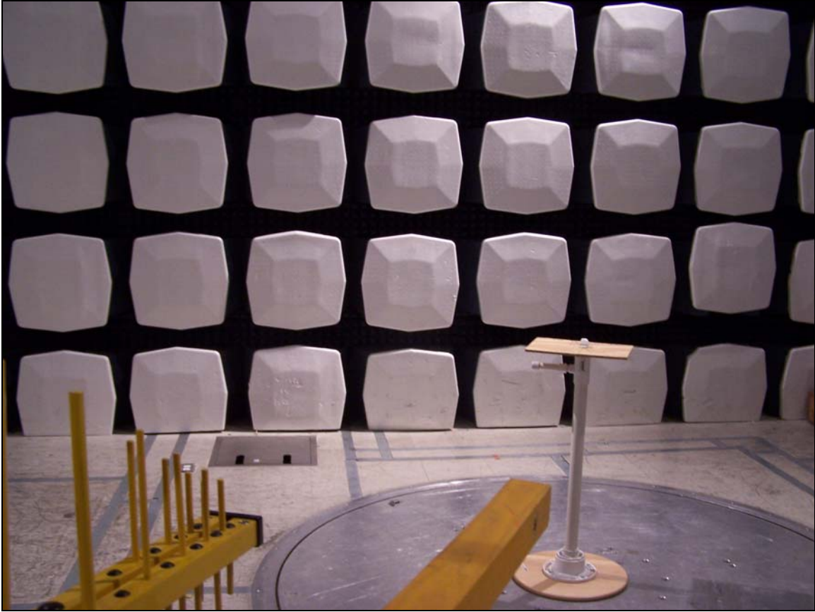
Photograph 1. Radiated Emissions Test Setup
