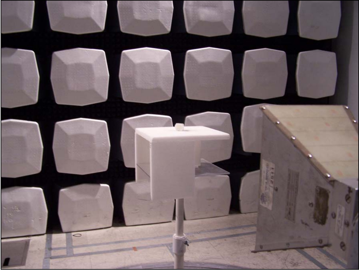
Photograph 5. Peak Test Setup
