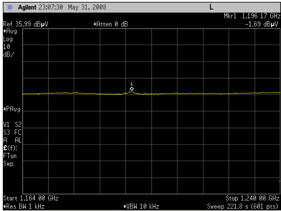
Plot 13. GPS, Band 1, T651-MIC (102-214)
