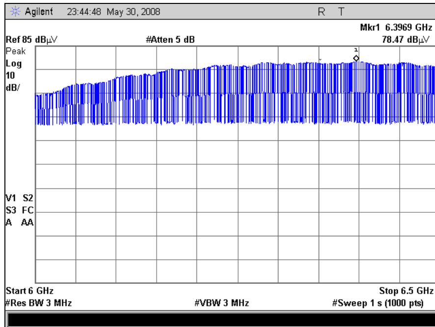
Plot 15. Peak Emissions, 6 – 6.5 GHz
