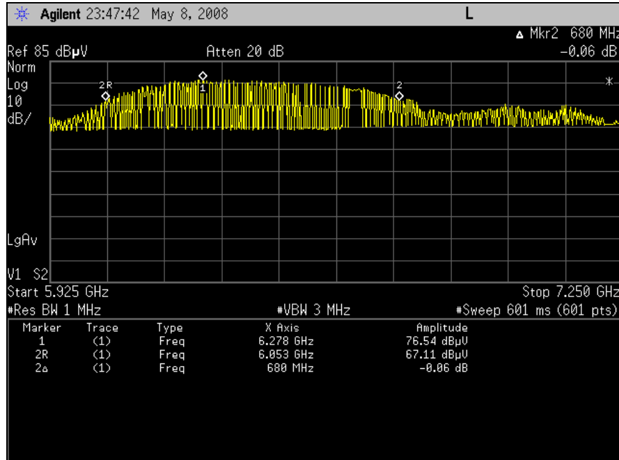
Plot 1. -10 dB Bandwidth, T651-MIC (102-214)
