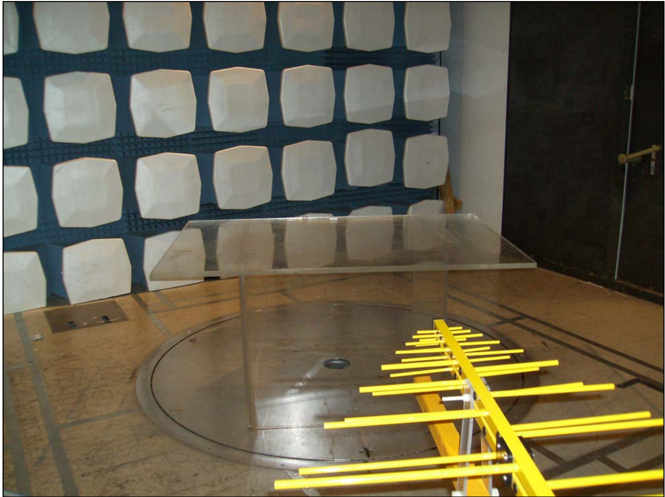
Photograph 4. Radiated Emissions Below 960 MHz, Test Setup
