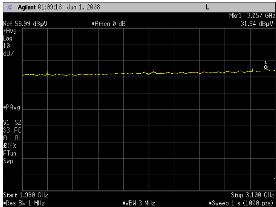
Plot 4. Emissions Above 960 MHz, Scan 3
