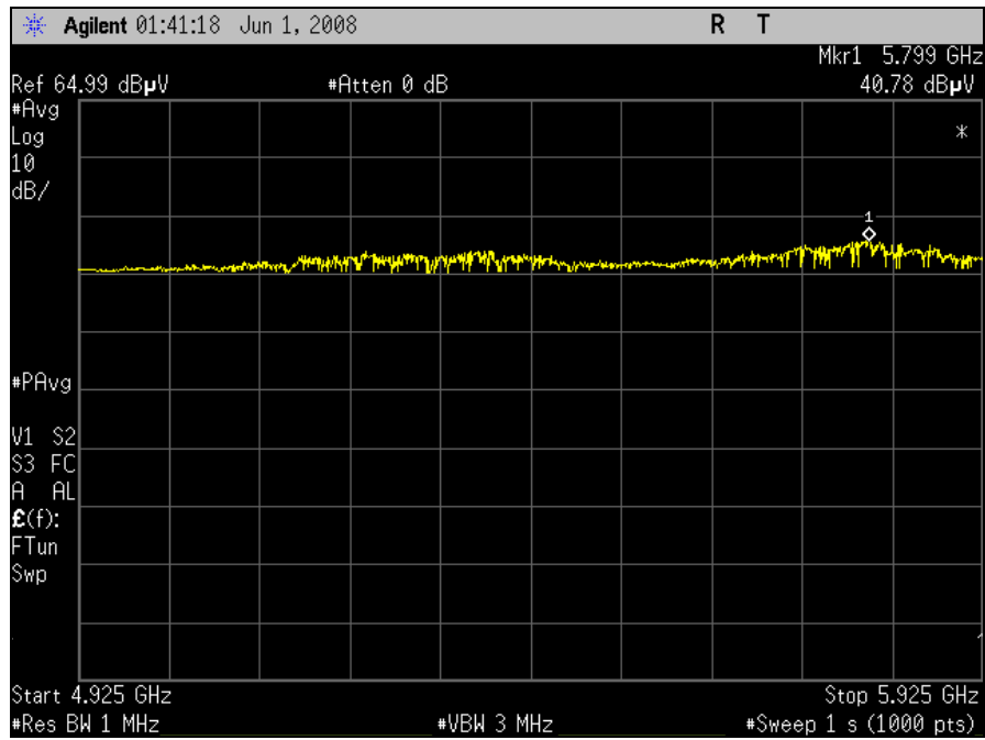
Plot 6. Emissions Above 960 MHz, Scan 5
