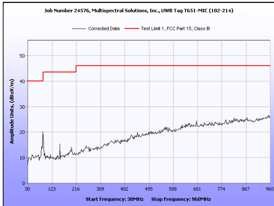
Plot 16. Emissions Below 960 MHz, T651-MIC (102-214)
