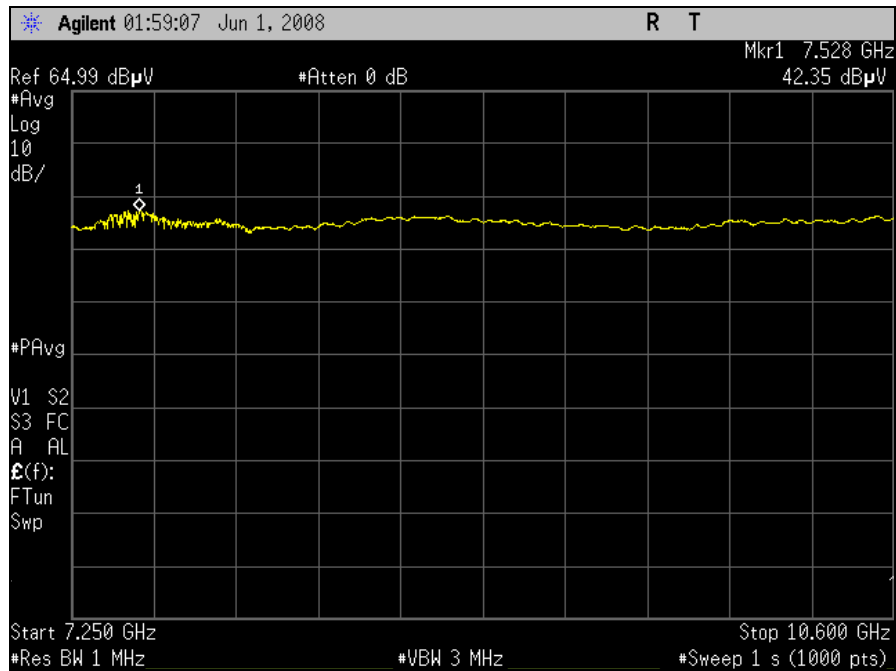
Plot 8. Emissions Above 960 MHz, Scan 7
