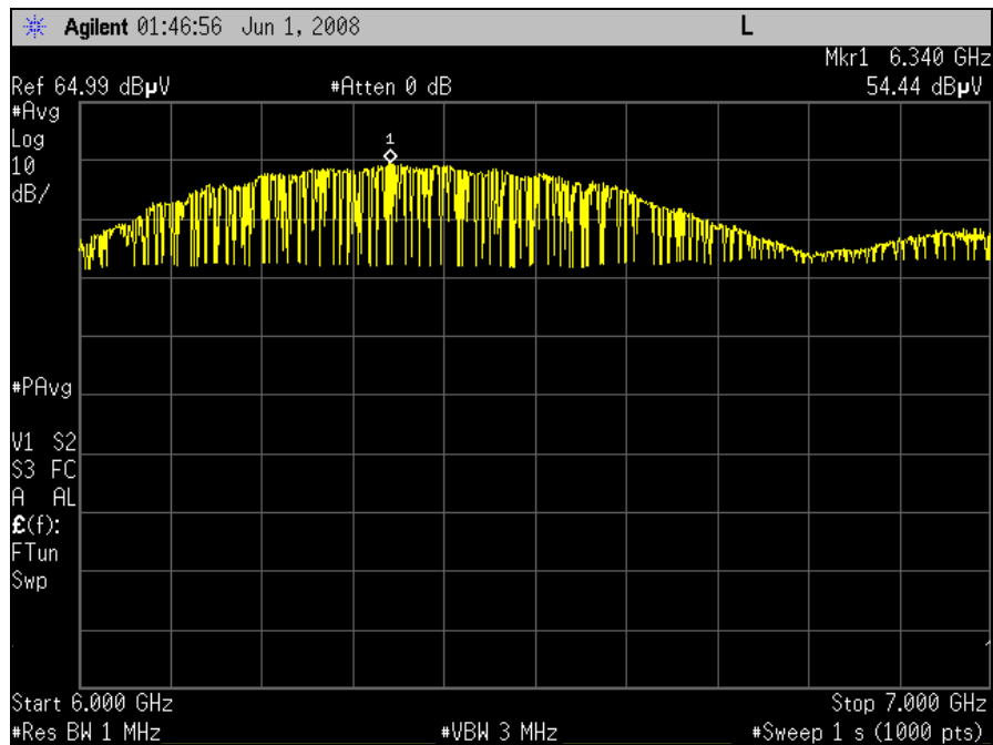
Plot 7. Emissions Above 960 MHz, Scan 6
