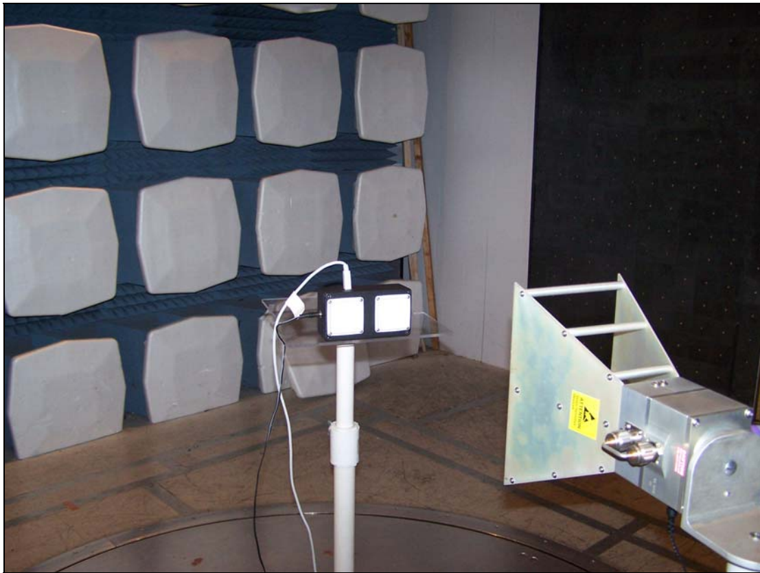
Photograph 3. Radiated Emissions Requirements, Broadband Test Setup
