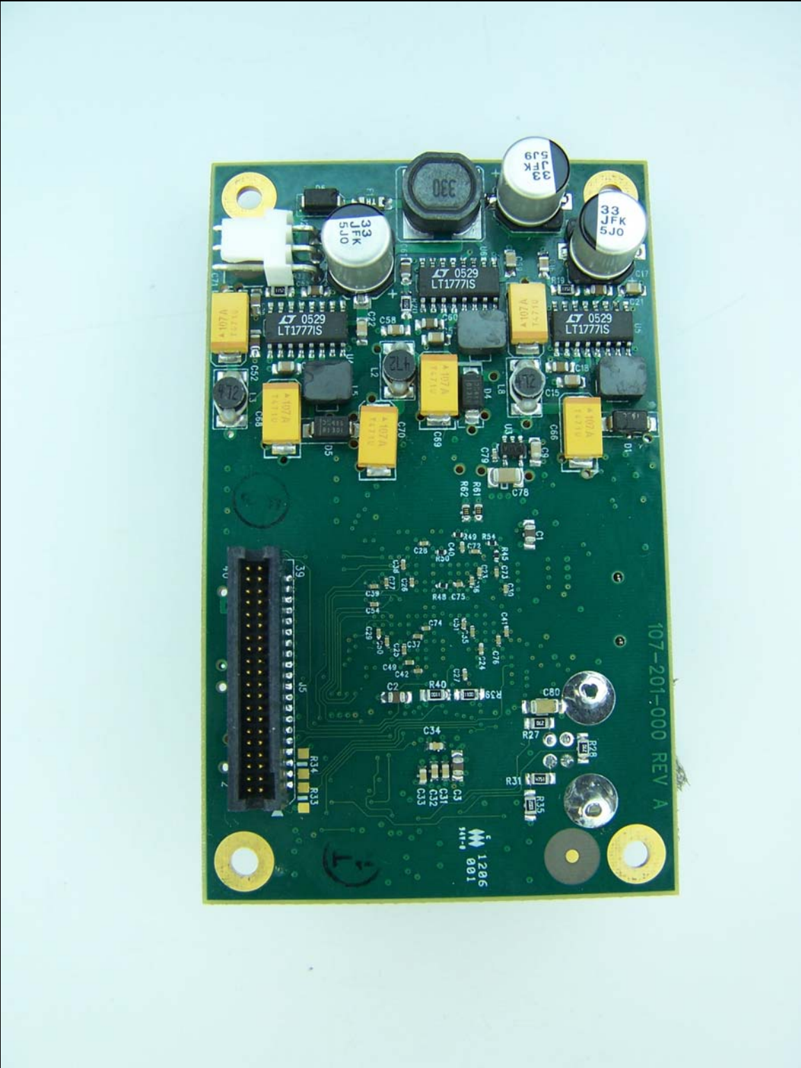
Photograph 9. View of Internal Components
