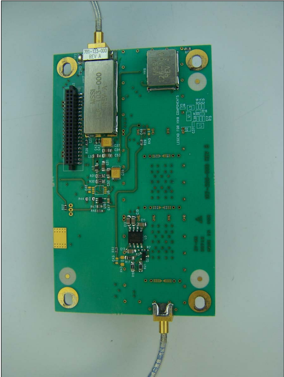
Photograph 10. View of Internal Components
