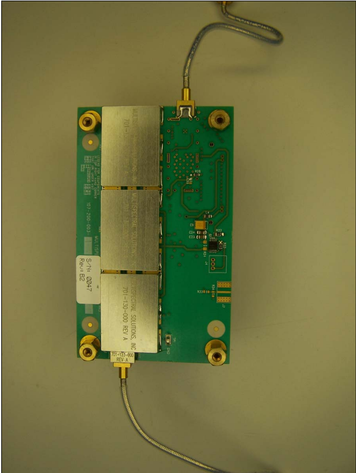
Photograph 8. View of Internal Components
