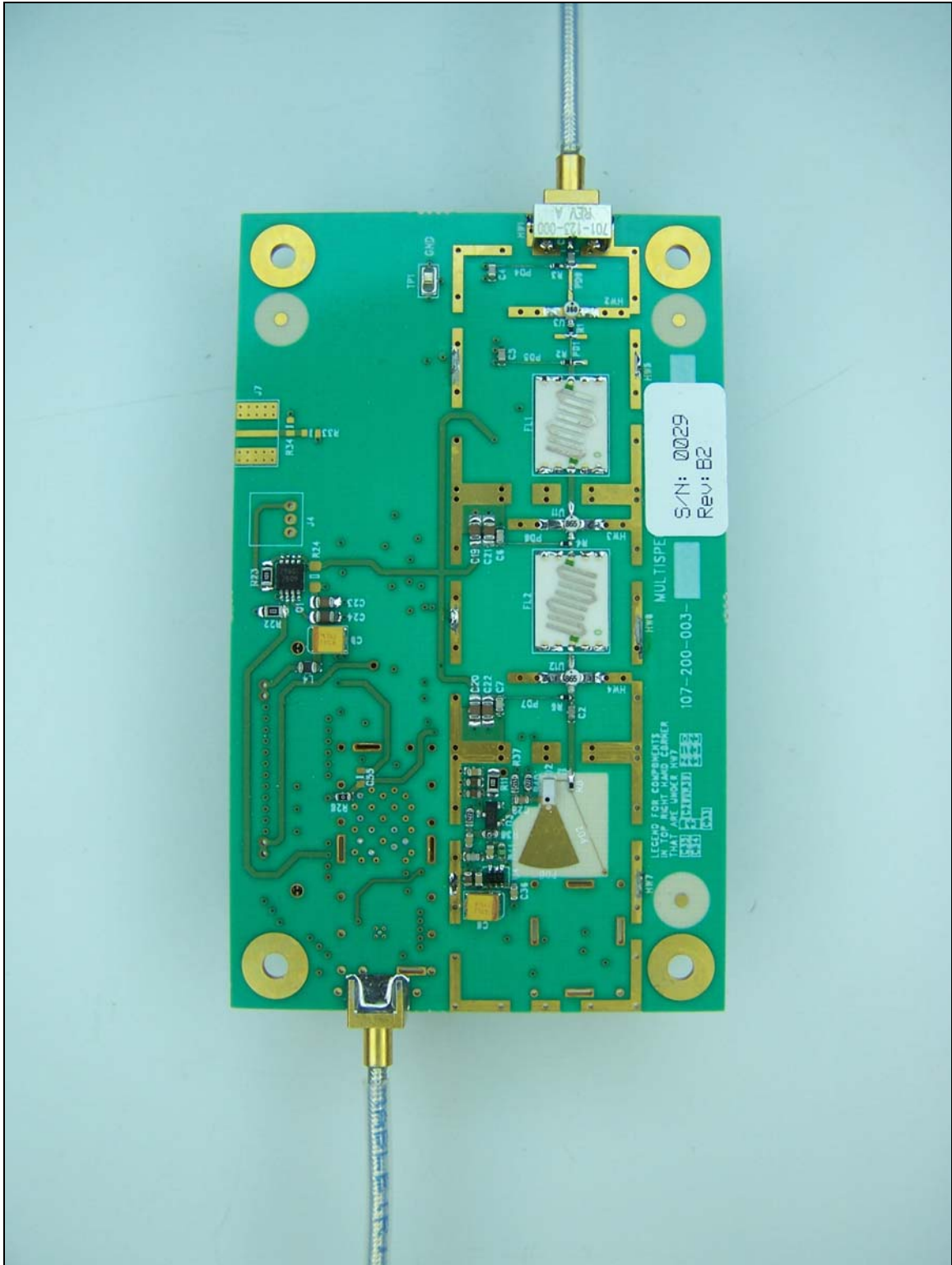
Photograph 12. View of Internal Components
