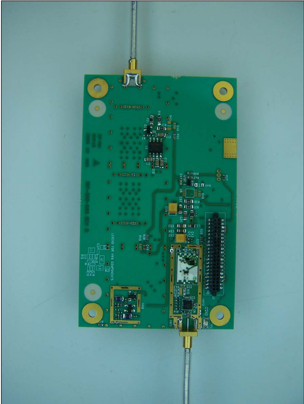
Photograph 4. View of Internal Components
