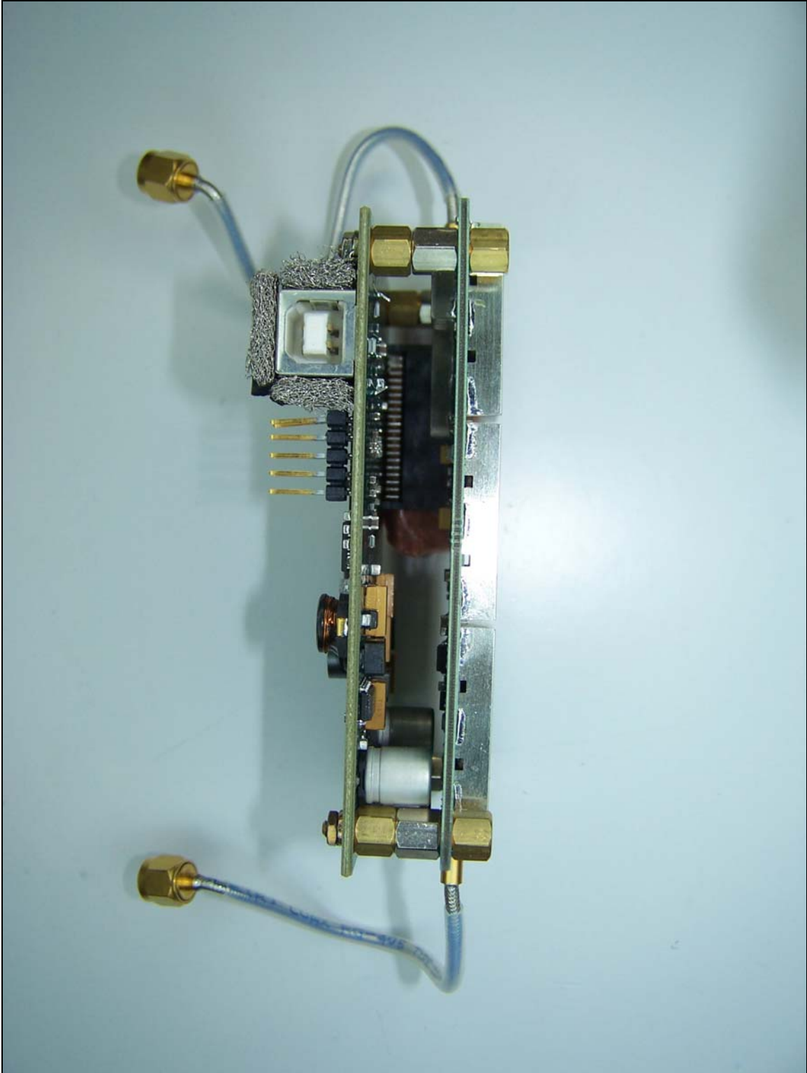
Photograph 7. View of Internal Components
