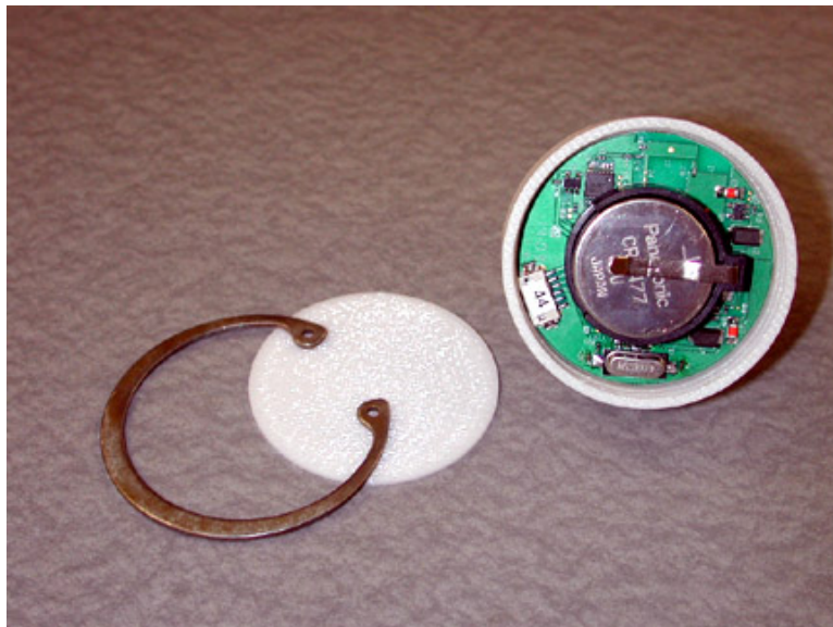
PAL-650 Disassembled
