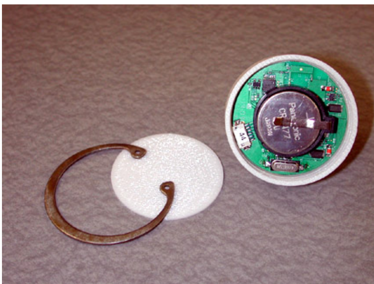
PAL-650 Disassembled
