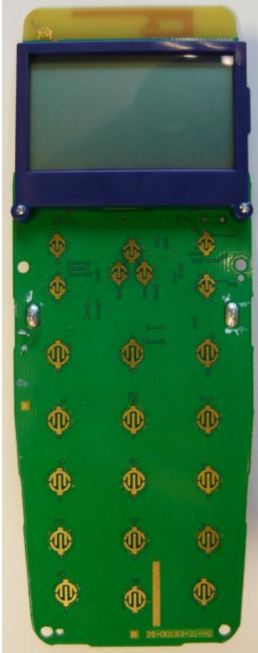
Top of PCBA after disassembly from top cover.
