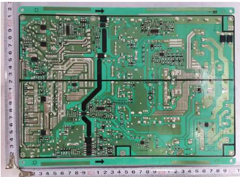
Power Supply (Soldering View)
