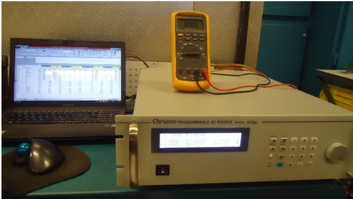
Figure 1.7 - Test Setup - Power system
