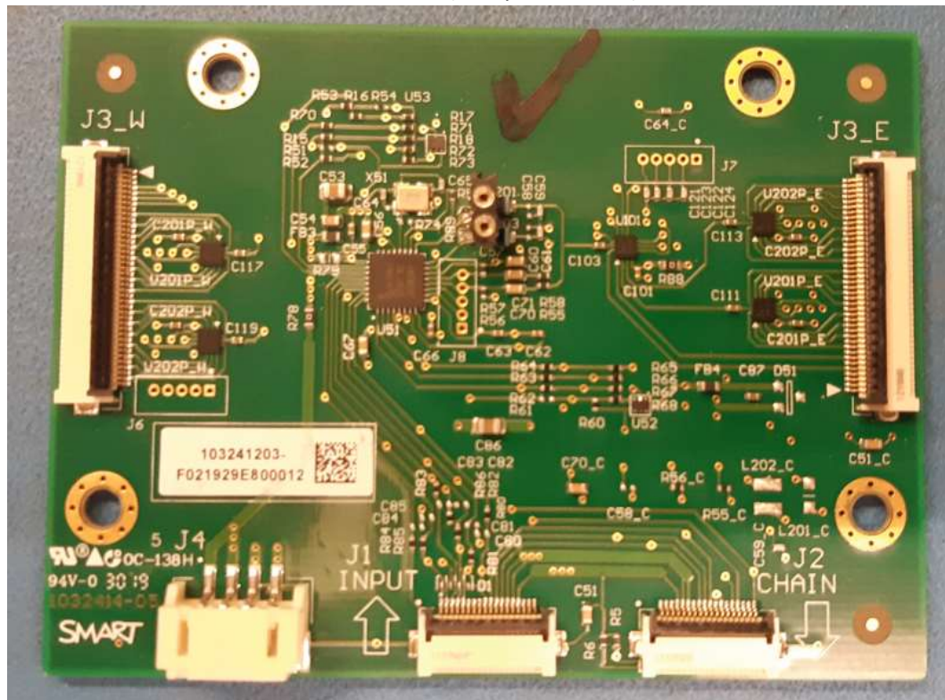
Kansas ISM (Component Side)
