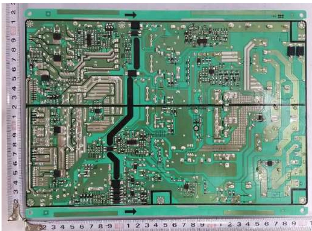
Power Supply (Soldering View)
