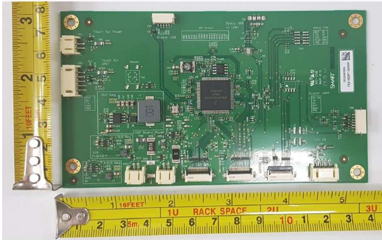
Kansas Touch Controller (Component Side)
