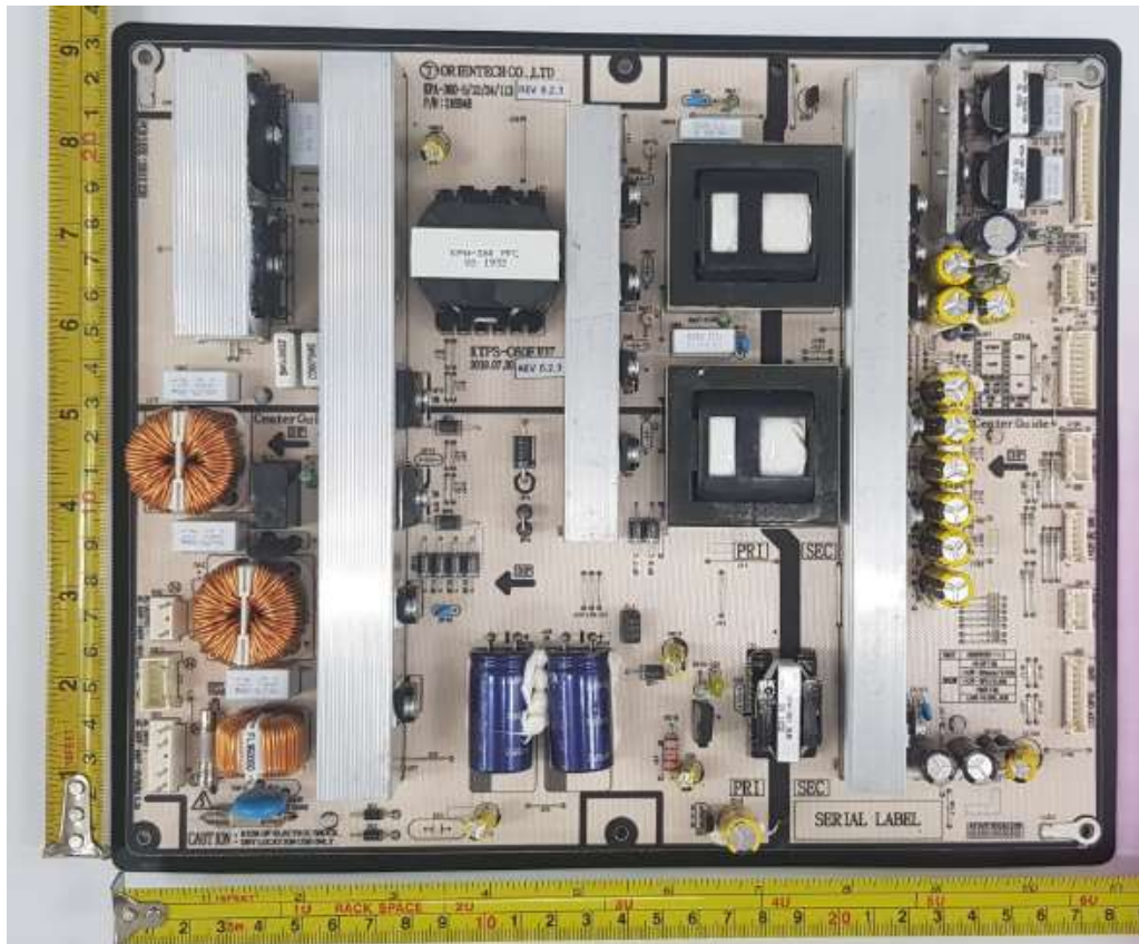
Power Supply (Component View)
