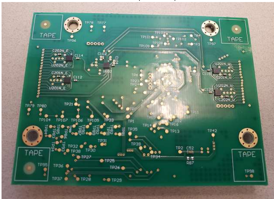
Kansas ISM (Solder Side)
