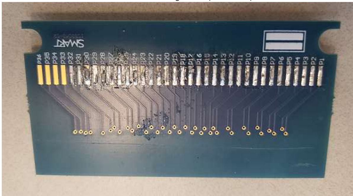
Kansas Matching boards (Solder Side)
