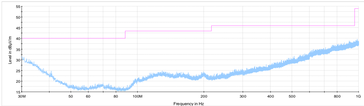
Figure 8.3-7: Radiated spurious emissions for mid channel below 1 GHz for restricted band emissions
