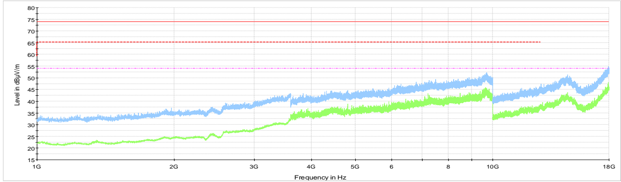
Figure 8.3-9: Radiated spurious emissions for low channel above 1 GHz for restricted band emissions
