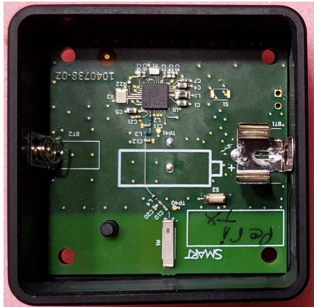
Battery Removed
