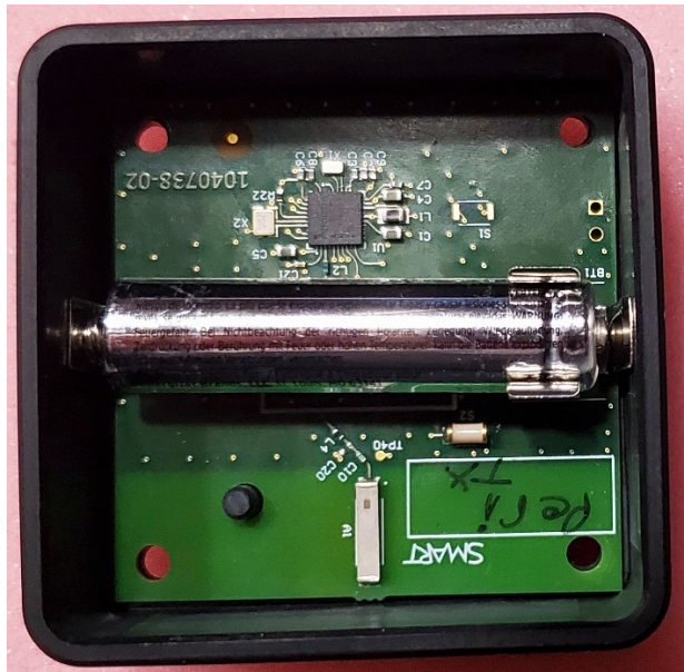
Top Removed
