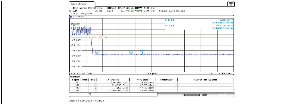
DH5_Ant1_High_Hop_2480
